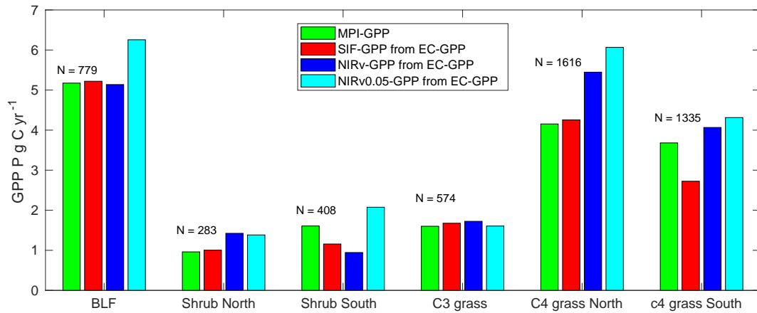
Figure 6. Comparison of aggregated MPI-BGC GPP, SIF-GPP and NIRv-GPP and GPP estimated from high resolution NIRv (NIRv0.05-GPP) for major biomes in Africa. N is the number of grid box of size 0.5^\circ \times 0.5^\circ used in the aggregation.
