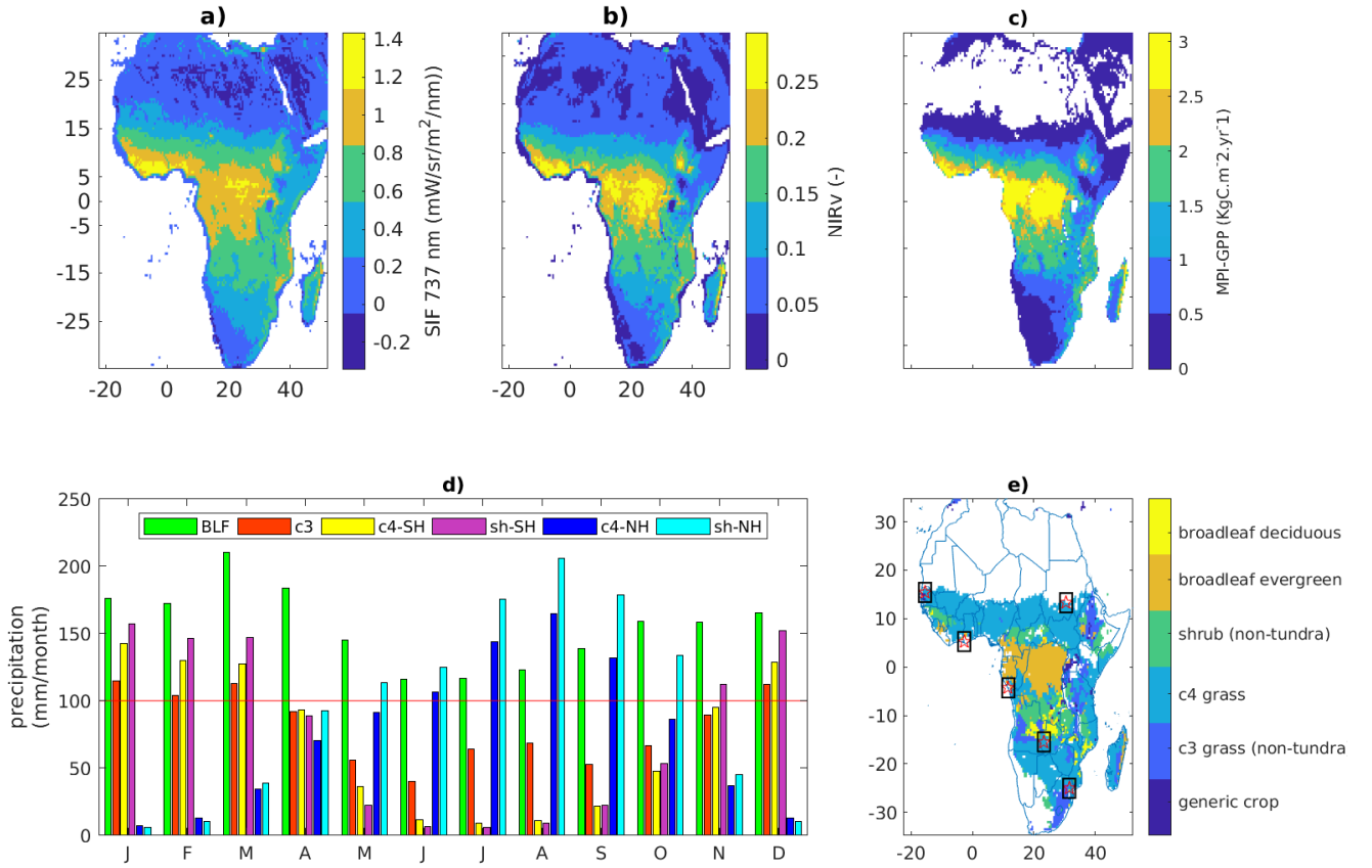
Figure 1. Annual mean SIF (a) and NIRv (b) averaged over the years 2007 – 2016 at 0.5^{\circ} \times 0.5^{\circ} resolution. (c) Climatology of gross primary production (Beer et al., 2010) at 0.5^{\circ} \times 0.5^{\circ} resolution. (d) Monthly average precipitation computed from the GPCC product covering the period from 1951 to 2000 for the major biomes of Africa. The red line indicates a reference of 100 mm/month. (e) Vegetation types from the terrestrial biosphere model SiBCASA. The white color refers to none vegetated regions. The rectangular window with a pentagon star at the center shows the distribution of flux towers in Africa.
