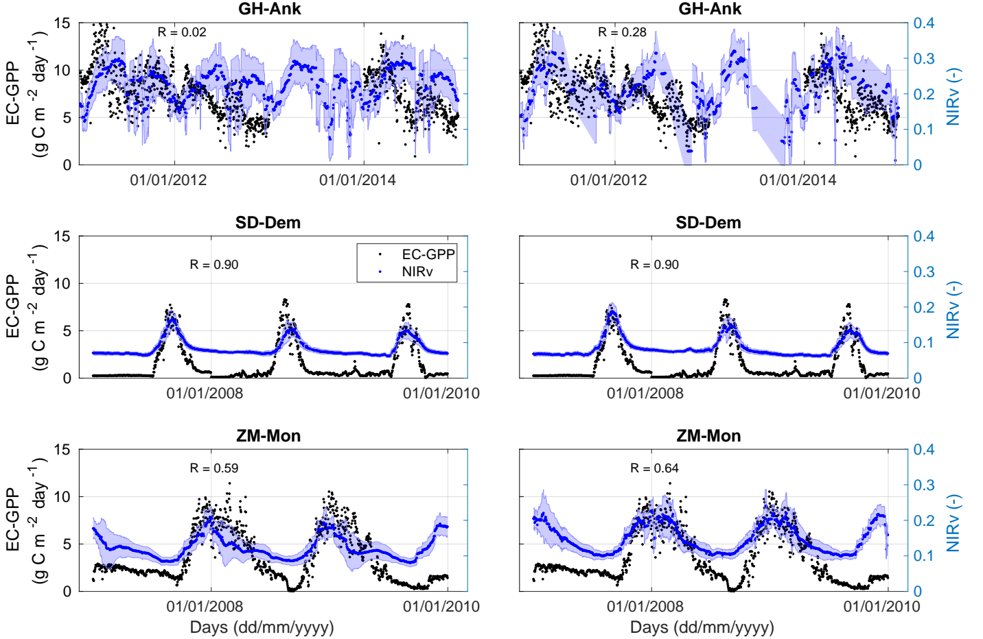
Figure 3. Comparison of coarse NIRv at 0.5^\circ \times 0.5^\circ (left panels) and high resolution NIRv at 0.05^\circ \times 0.05^\circ (right panels) with flux tower measured GPP (EC-GPP) for a selection of three African flux towers (GH-Ank, SD-Dem and ZM-Mon). The temporal correlation between NIRv and EC-GPP is given in each panel.
