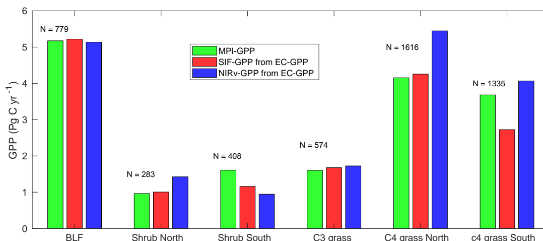
Figure 6. Comparison of aggregated MPI-BGC GPP, SIF-GPP and NIRv-GPP for major biomes in Africa. N is the number of grid box of size 0.5^\circ \times 0.5^\circ used in the aggregation.
