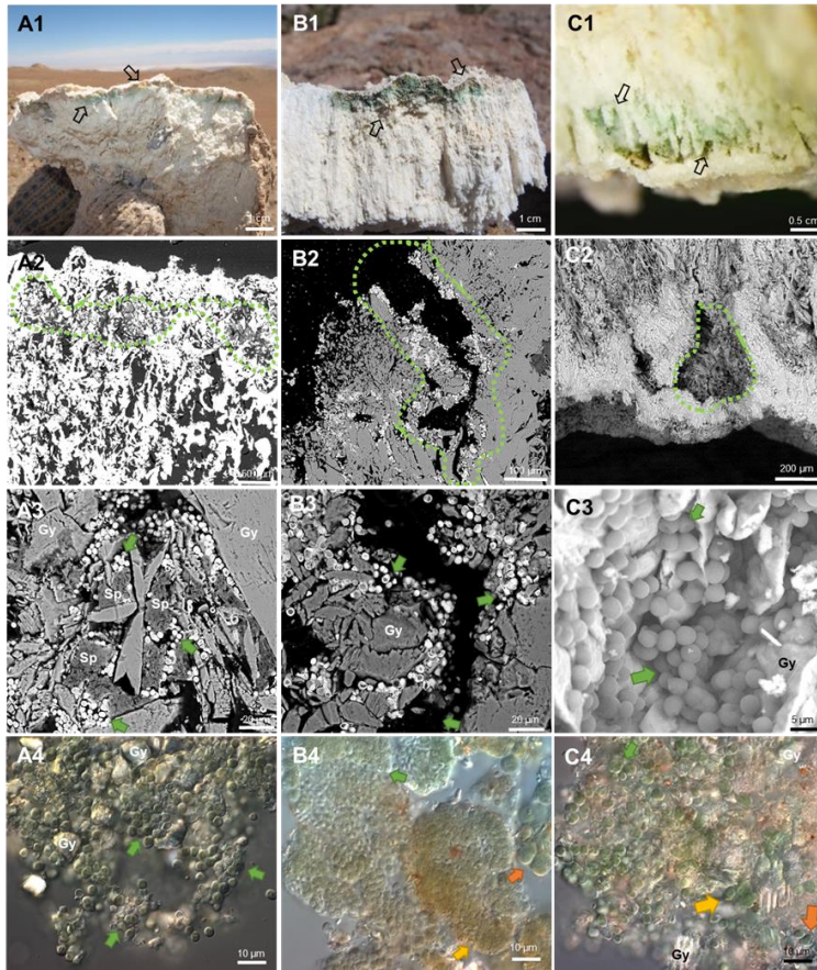
Figure 3: Endolithic colonization zones characterization. Series A: Cryptoendolithic; Series B: Chasmoendolithic; Series C: Hypoendolithic. Series 1: Macro images of gypcrete cross-section of colonized zones; Series 2 and 3: SEM-BSE images of gypcrete cross-section of colonized zones; Series 4: LM-DIC images of scrapped cyanobacteria from gypcrete. Series 1: Black arrows indicate green and orange coloured endolithic colonization zones of 5 mm thick on A1 (CR), 8 mm thick on B1 beneath the surface (CH) and 5-9 mm thick on C1 above bottom gypsum crust (HE). Series 2. CR, CH and HE microhabitats with aggregates of endolithic microbial communities surrounded by the green dotted lines, inside the pores of gypcrete: A2, under a white dense surface crust; B2, inside the cracks of gypcrete and C2, inside the micro caves of gypcrete at bottom of the rock. Series 3 Green arrows point to aggregates of cyanobacteria among gypcrete (Gy) crystals (A3, B3), surrounding by sepiolite (Sp) nodules (A3) and on the gypcrete (Gy) walls (C3). Series 4 aggregates of different morphotypes of cyanobacteria, shown by green, yellow and orange arrows and gypcrete crystals (Gy).
