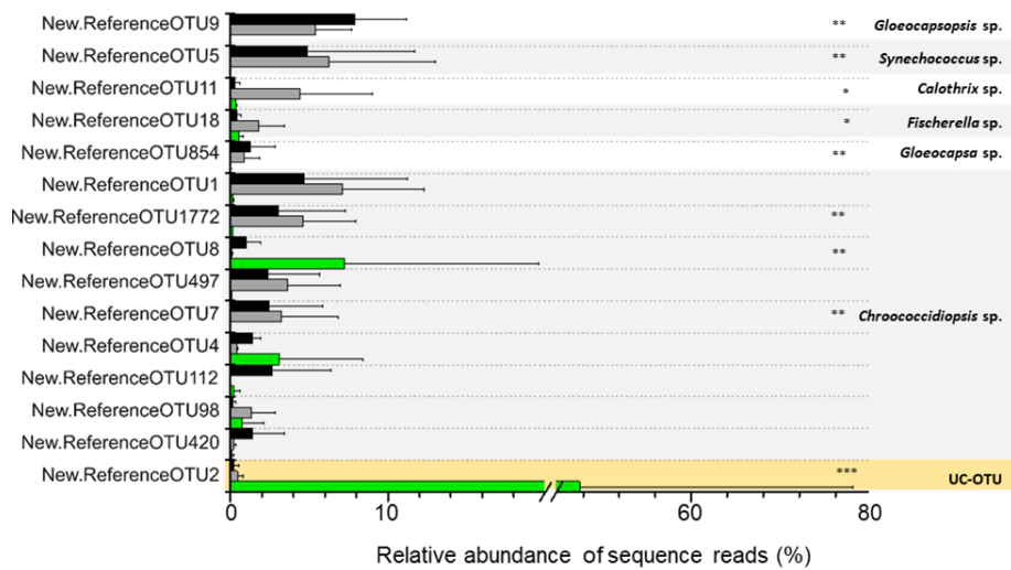
Figure 6: Average relative abundance of cyanobacterial OTUs. Differentially abundant cyanobacterial OTUs across the three microhabitats are represented by *(Diff-OTUs p -value <0.01 Ch / Cr-He), ** (Diff-OTUs p -value <0.001 He / Cr-Ch), *** (Diff-OTUs p -value <0.0001 He / Cr-Ch). UC-OTU (Unclassified Cyanobacterial OTU). Only sequences > 1\% relative abundances were used.
