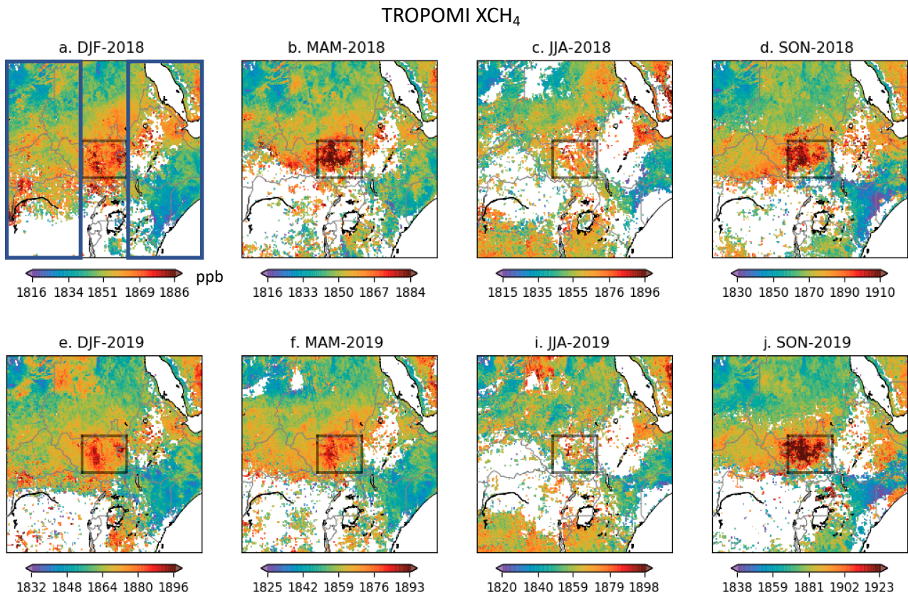
Figure 2. Seasonally average TROPOMI XCH 4 (ppb) at 0.1^\circ \times 0.1^\circ resolution. The black rectangle at the centre of each panel shows the SSWR source region. The area outside of it is used as the background region. XCH 4 is corrected for large-scale latitudinal variation by subtracting a 3 rd order polynomial fit using the region shown by blue rectangles in panel a. The region excludes the longitudes of the source region. Note that DJF includes December of the previous year.
