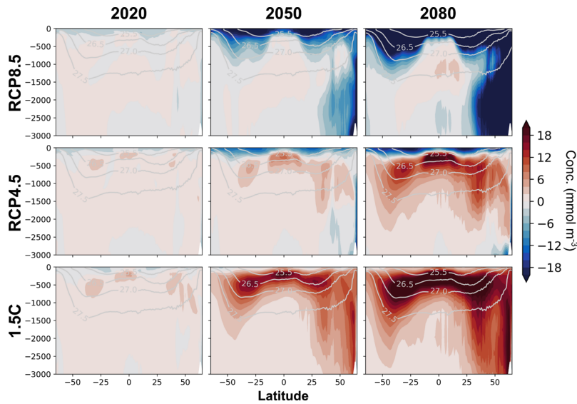
Figure 4. Ocean component model output of the global zonal mean deviation of anthropogenic carbon concentration ( \text{mmol m}^{-3} ) from the historical scaling of anthropogenic carbon ( C_{ant}^* - C_{ant} ). Rows and columns same as Figure 1. Positive regions indicate faster carbon accumulation than historical scaling, negative regions indicate slower accumulation. Contour lines are surfaces ( \text{kg m}^{-3} ).
