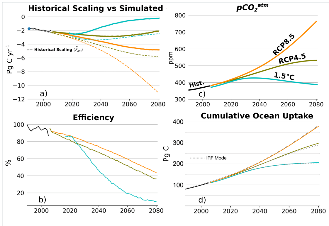
Figure 2. (a) Historical scaling of ocean anthropogenic carbon uptake ( F_{ant}^* ; dotted lines) and CEM3 anthropogenic carbon uptake ( F_{ant} ; solid lines) for three scenarios (1.5°C, RCP4.5, and RCP8.5). Negative indicates atmospheric anthropogenic carbon removal. (b) Efficiency of the global ocean sink for the three scenarios from CEM3 (Equation 5). (c) p\text{CO}_2^{atm} for both CEM3 and IRF model. (d) Total anthropogenic carbon accumulation in CEM3 (solid lines) and in the IRF model (dotted lines). Flux and efficiency from 2006-2017 are not shown for 1.5°C scenario due to ocean adjustment to p\text{CO}_2^{atm} forcing (see Methods 2.2; Figure S2).
