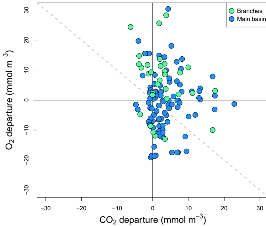
760 Figure 5: Surface O 2 versus CO 2 departure from saturation for all sampled surface sites in the reservoir main basin and branches across all sampling campaigns.
