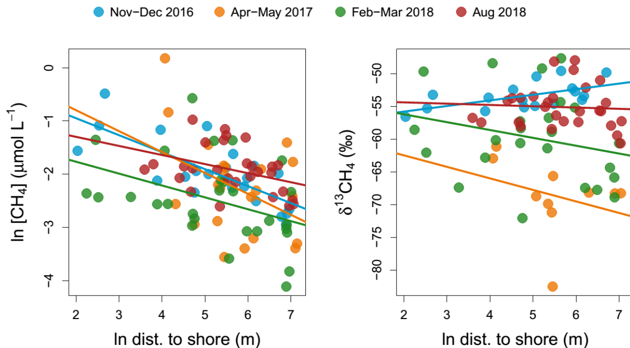
765 Figure 6: Regression of \text{CH}_4 concentration (left panel) and isotopic signature (right panel) as a function of distance to shore in each sampling campaign in the main reservoir basin. For \text{CH}_4 concentration, regressions lines have the following statistics in order of sampling: p-values: < 0.001 , 0.06 , 0.03 , 0.05 , and R^2_{\text{adj}} : 0.54 , 0.13 , 0.11 . For \delta^{13}\text{CH}_4 , all regressions had p-values > 0.2 except for the Nov-Dec 2016 campaign with p-value = 0.01 and R^2_{\text{adj}} = 0.29 .
