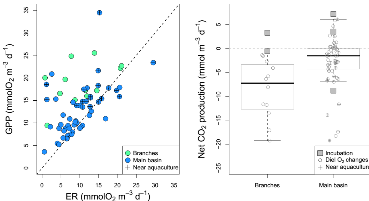
755 Figure 4: Epilimnetic daily GPP versus ER rates (left panel) derived from diel \text{O}_2 changes in the reservoir branches and main basin (including sites near aquacultures), with the 1:1 line (dotted). Boxplots of the corresponding rates of \text{CO}_2 NEP (right panel) in the branches and main basin, with boxes bounds, whiskers, solid line, and open circles, and squares representing the 25th and 75th percentiles, the 10th and 90th percentiles, the median, single data points (diel \text{O}_2 method), and incubation derived rates respectively.
