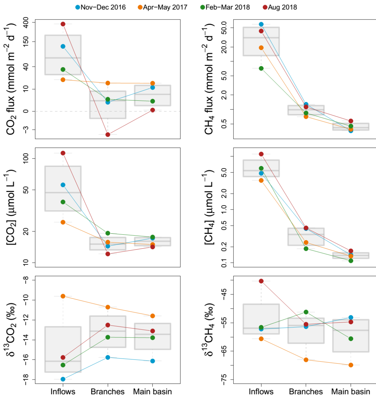
745 Figure 2: Average of spatially interpolated surface CO 2 and CH 4 fluxes, concentrations, and isotopic signatures along the hydrological continuum from the reservoir inflows to the main basin for each sampling campaign.
