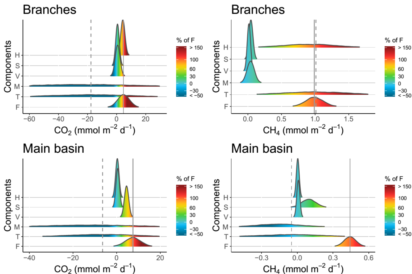
750 Figure 3: Density distributions of the different components of CO 2 and CH 4 surface budget in the reservoir branches and main basin (H = horizontal flow inputs, S = sediment inputs, V = vertical inputs, M = net metabolism, T = sum of all estimated sources and processes in the surface layer, and F = measured surface fluxes). Density curves are based on simulated normal distributions using the mean and standard error of each component. The color scale represents the percentage of the mean surface flux accounted by each component. The solid and dashed grey lines represent the means of F and T respectively.
