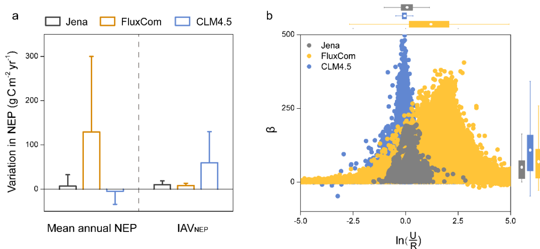
Figure 1A. Representations of the spatially varying NEP and its local indicators in FLUXCOM product and the Community Land Model (CLM4.5) at the global scale. a , The variation of mean annual NEP and IAV_{NEP} derives from Jena Inversion, FLUXCOM and CLM4.5. Variation in mean annual NEP: the spatial variation of mean
