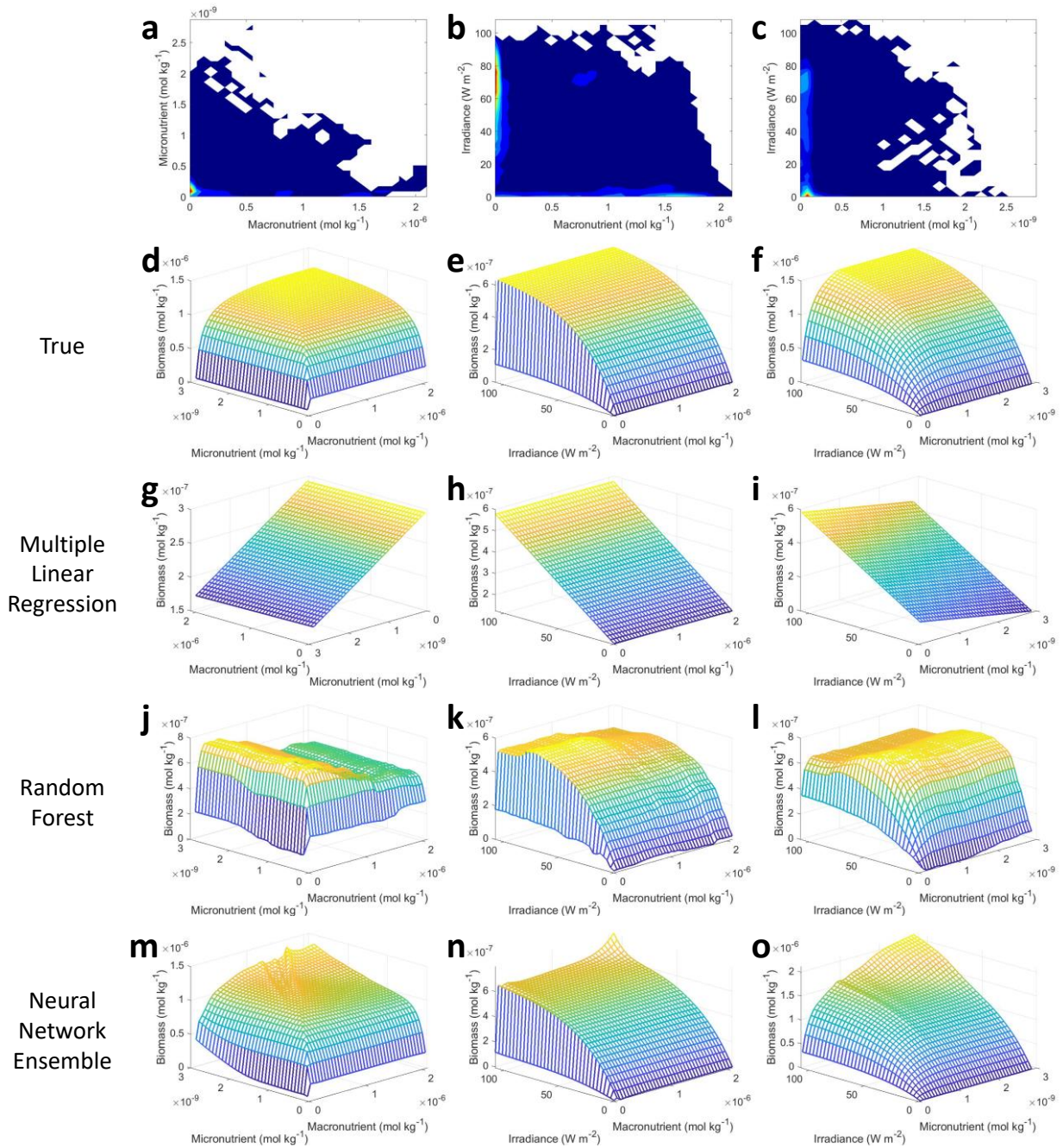
1127 Figure 3: Contour and interaction plots for Scenario 1. The contour plots show the density of observations for each 1128 set of predictors (a-c) where blue signifies very few observations and colors moving up the spectrum to red indicate 1129 many observations. The interaction plots (d-o) show the biomass values for different combinations of the predictors 1130 on each x and y axis. The predictor that was not varying was set at its 50 th percentile (median) value (ex. Subplot d 1131 allows the micro- and macronutrient to vary across their respective min-max ranges, while the irradiance is held 1132 fixed at its 50 th percentile value). The top three interaction plots (d-f) show the true interactions calculated from Eq. 1133 1-3. The remaining interaction plots show the predicted interactions for MLR (g-i), RF (j-l), and NNE (m-o). Note
