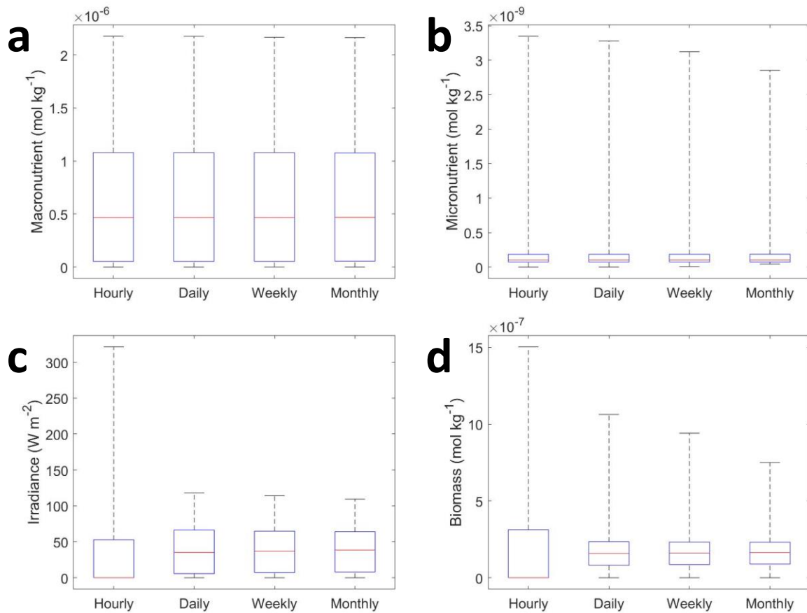
1161 Figure 6: Boxplots showing the variability in the predictor and target variables of Scenario 2 for the various time- 1162 averaged datasets. The predictor variables include (a) macronutrient, (b) micronutrient, and (c) irradiance. The target 1163 variable was phytoplankton (d) biomass. The red line corresponds to the median (50 th percentile), the box edges are 1164 the 25 th and 75 th percentile values, and the whiskers are the minimum and maximum values.
