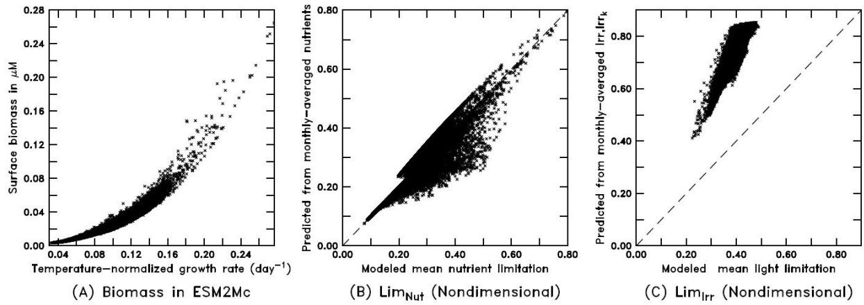
1195 Figure 10: Scatter plots from the BLING model (a: surface biomass vs. temperature-normalized growth rate; b: 1196 monthly-averaged nutrients vs. mean nutrient limitation; c: monthly-averaged Irr, Irr k vs. mean light limitation).
