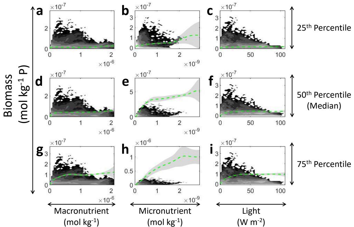
1199 Figure 11: Sensitivity analysis for Scenario 3 showing the predicted relationships for the NNE. The columns 1200 correspond to the predictors and the rows correspond with the percentile value at which the other predictors were set 1201 (ex. Subplot a varies the macronutrient across its min-max range, while the micronutrient and light are held at their 1202 25 th percentile values, respectively). The green dashed line shows the apparent relationships predicted by the NNE. 1203 The predicted relationships are the average of the individual predictions for each NN. The gray regions around the 1204 NNE dashed lines show one standard deviation in the predictions (ex. One standard deviation in the 10 individual 1205 NN predictions of the NNE). The contour plot behind the predicted relationships show the observations for each 1206 predictor against the biomass. Lighter colors signify a higher density of observations, while darker colors correspond 1207 to fewer observations.
