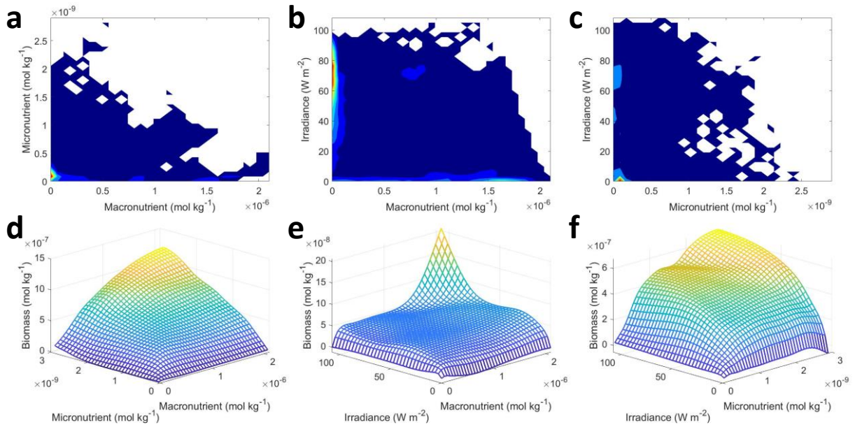
1209 Figure 12: Contour and interaction plots for Scenario 3. The contour plots show the density of observations for each 1210 set of predictors (a-c) where blue signifies very few observations and colors moving up the spectrum to red indicate 1211 many observations. The interaction plots (d-f) show the biomass values for different combinations of the predictors 1212 on each x and y axis. The predictor that was not varying was set at its 50 th percentile (median) value (ex. Subplot d 1213 allows the micro- and macronutrient to vary across their respective min-max ranges, while the irradiance is held 1214 fixed at its 50 th percentile value). The interaction plots show the predicted interactions based on the NNE. The 1215 predicted relationships are the average of the individual predictions for each NN.
