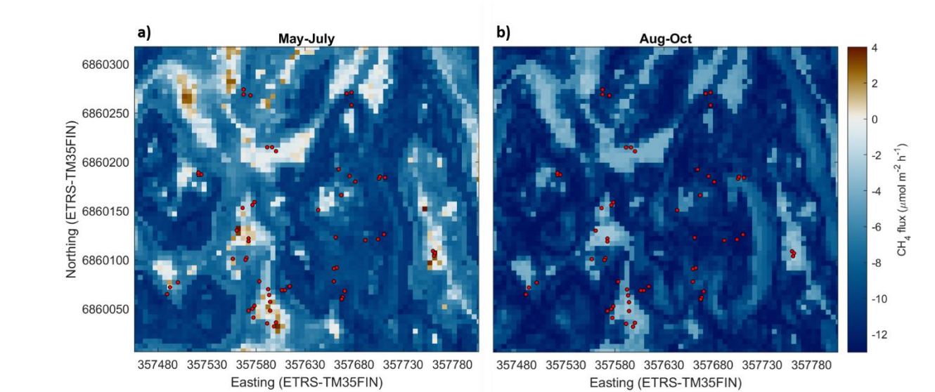
Figure 8. Modelled forest floor CH 4 flux ( \mu\text{mol m}^{-2} \text{h}^{-1} ) at the site in May–July (a) and August–October (b). (Values below zero indicate uptake and values above zero emission). The red circles show the sample points.
