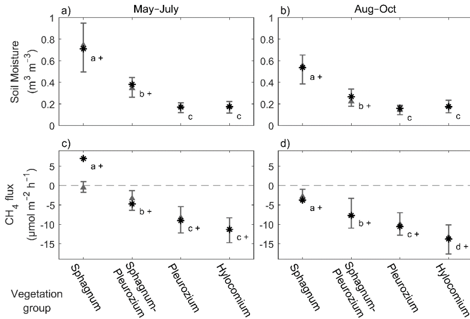
385 Figure 4. The soil moisture (volumetric water content, \text{m}^3 \text{m}^{-3} ) (a, b) and the measured \text{CH}_4 flux ( \mu\text{mol m}^{-2} \text{h}^{-1} ) (c, d) of the different vegetation groups in May–July and August–October. The asterisks indicate the mean values, triangles indicate the medians, and the whiskers show the 25 th and 75 th percentiles. Statistically significant differences ( p < 0.05 ) within each subplot are marked with different letters, and plus signs indicate significant differences between the seasons in a group. Sample points in the Sphagnum group have >50\% cover of Sphagnum sp., while Hylocomium group sample points have typically \geq 80\% of Hylocomium splendens , and the others are intermediary groups between the extremes.
