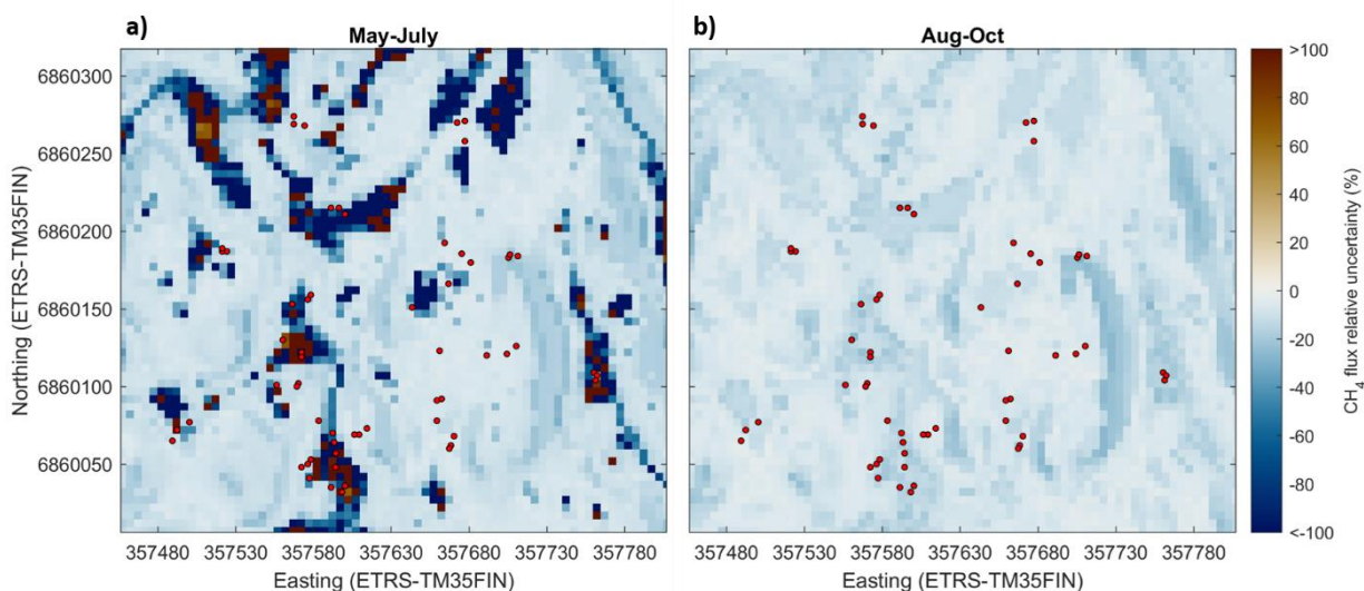
Figure 9. Relative uncertainty of the modelled forest floor CH 4 flux (%) at the site in May–July (a) and August–October (b). The relative uncertainty was defined as the standard deviation of the results of individual Random Forest models in the RF model ensemble divided by the modelled CH 4 flux (see Sect. 2.8). The red circles show the sample points.
