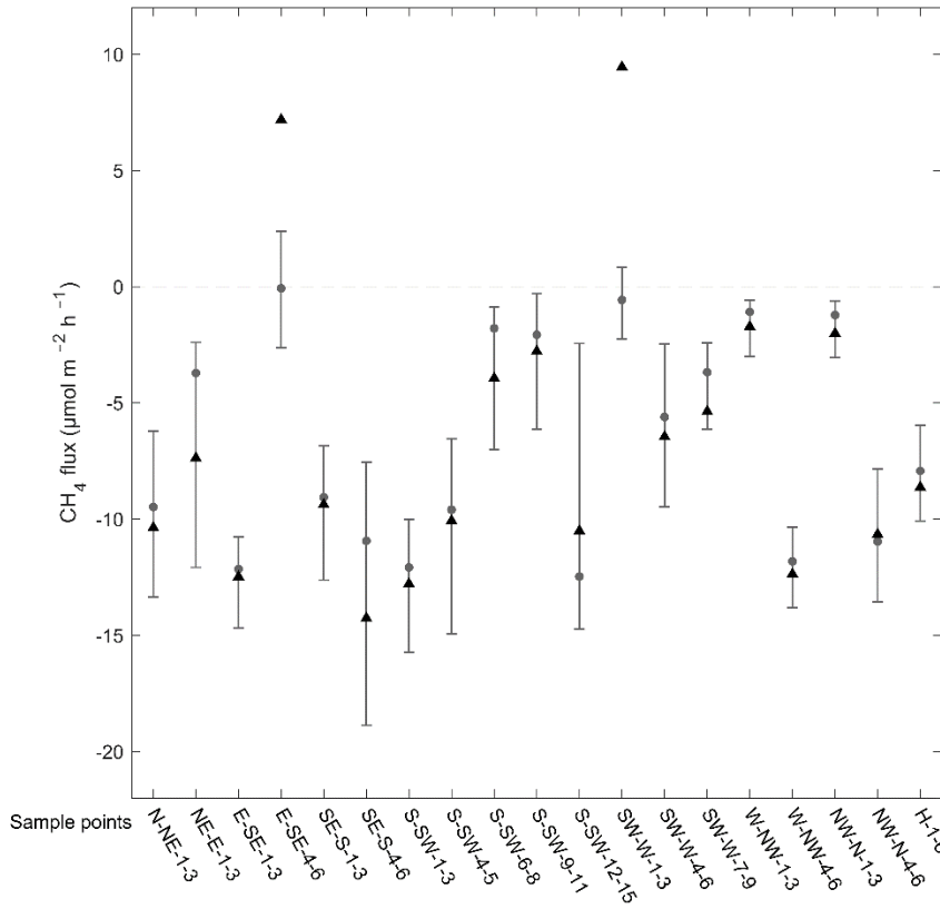
Figure 5. Fluxes of CH 4 ( \mu\text{mol CH}_4 \text{m}^{-2} \text{h}^{-1} ) from the sample point groups. Mean values are represented with triangles, medians with circles, and the whiskers show 25 th and 75 th percentiles.
