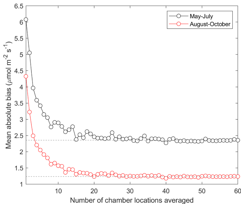
Figure 10. Mean absolute bias in the measured forest floor CH 4 flux estimated from a random subset of the sample points. Mean upscaled CH 4 flux was used as a reference. (Max. 500 sample point combinations were calculated.)
