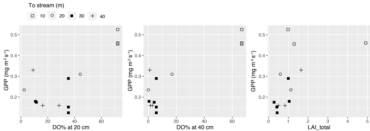
Figure A6: Gross primary production (GPP) at a photosynthetic photon flux density level of 800 \mu\text{mol m}^{-2}\text{s}^{-1} in the methane ( \text{CH}_4 ) flux sample plots in clusters 10–40 plotted against peak season (early summer) dissolved oxygen concentration (DO%) at 20 and 40 cm below the surface, and peak season (late July) total vascular leaf area index (LAI total ). Plots in the same cluster are labeled using the same symbol.
