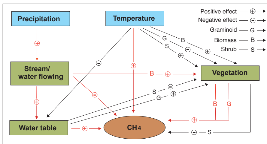
435 Figure 7: Schematic illustration showing the potential independent and interactive impacts of precipitation, temperature, vegetation and hydrology on methane (CH 4 ) fluxes in northern peatlands. Arrows in red and black are derived from this study and previous studies, respectively (e.g., Mäkiranta et al., 2018; Roulet et al., 1992; Yavitt et al., 2019).
