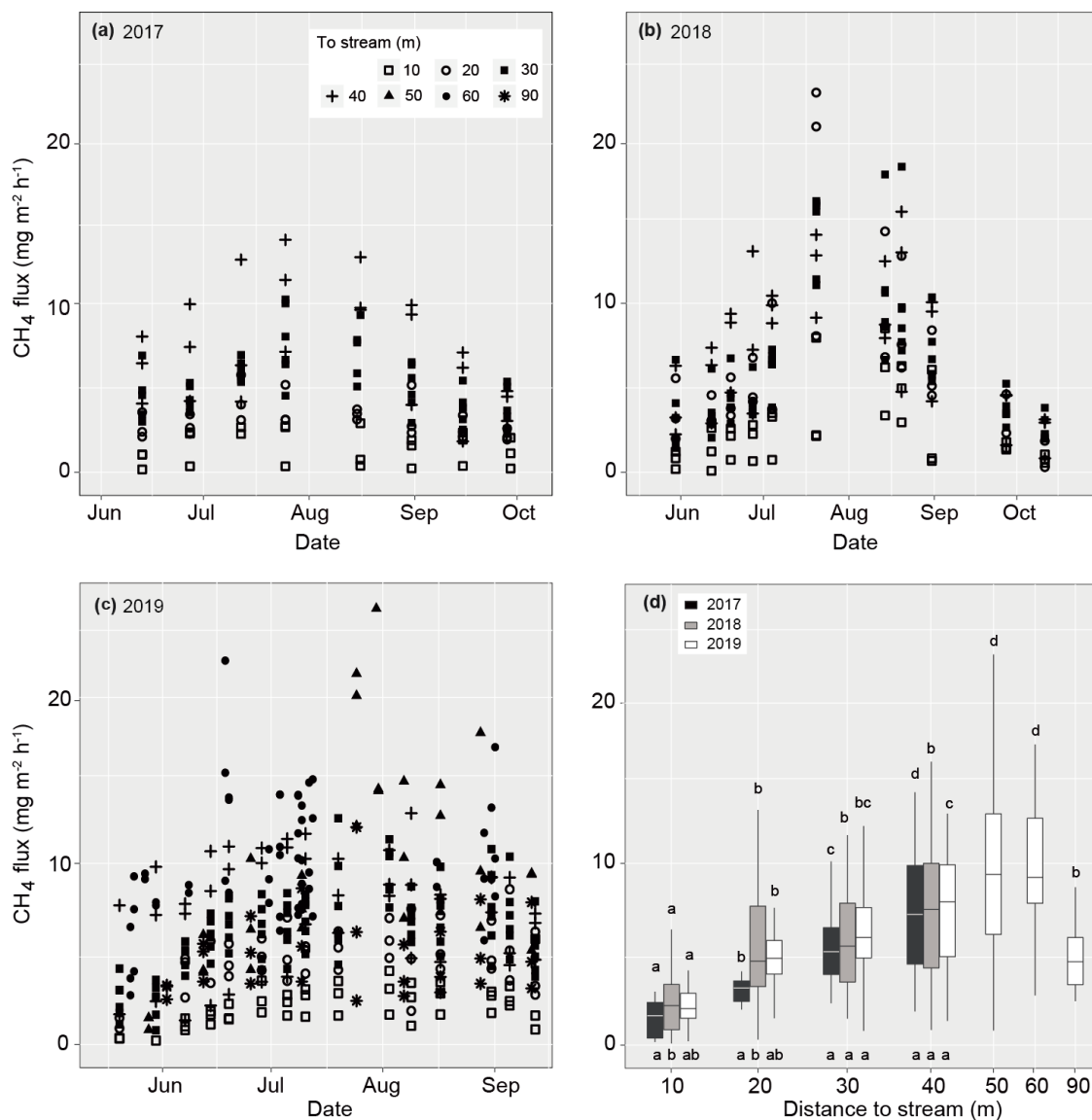
Figure 4: Measured methane (CH 4 ) fluxes during the growing season in (a) 2017, (b) 2018, and (c) 2019 at Lompolojänkä. Distance to the stream of the sample plot clusters are indicated by different symbols. (d) Box plots of CH 4 fluxes for each measurement cluster in 2017, 2018 and 2019. The different letters on top of the box plots indicate significant differences ( p < 0.05 ) between the clusters for each year, calculated using Tukey's Honest Significant Difference method, and the different letters below the box plots indicate significant differences ( p < 0.05 ) between the studied years for each cluster.
