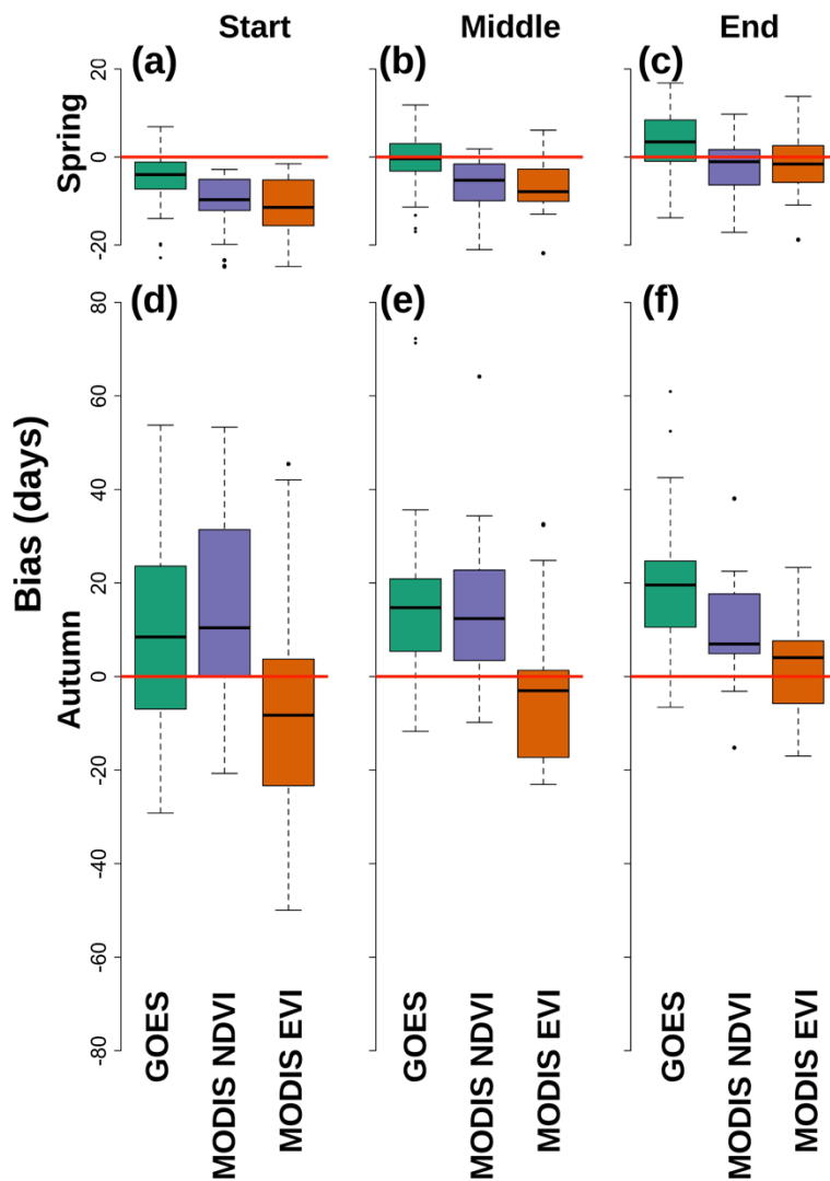
590 Figure 6: The different biases for the different satellite-based data sources compared to PhenoCam for their estimation of spring start (a), middle (b), and end (c); and autumn start (d), middle (e), and end (f). A negative bias indicates the given data source was earlier than PhenoCam. The red line denotes zero bias. Boxes are color coded by the data source as indicated on the x-axis. The biases are larger in the autumn than in the spring. There are some with little median bias.
