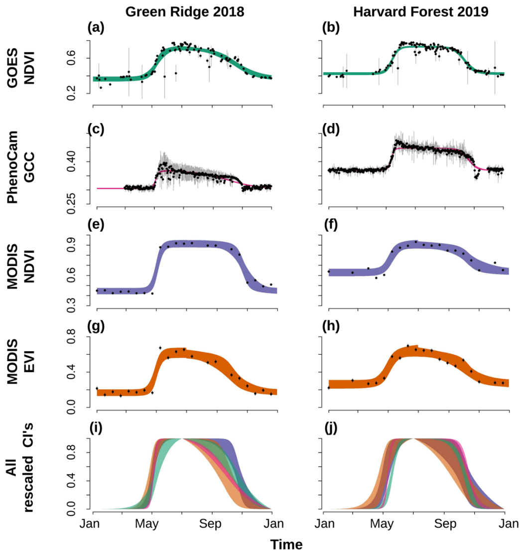
570 Figure 3: Timeseries of data from GOES NDVI daily data (a and b), PhenoCam GCC (c and d), MODIS NDVI (e and f), MODIS EVI (g and h) and the rescaled credible intervals (i and j) for Green Ridge 2018 (left column) and Harvard Forest 2019 (right column). (a–h) include mean observations in black dots with 95% confidence intervals shown with vertical gray lines. 95% credible intervals (CI) are given with the different shading specific to each data source. The Green Ridge 2018 spring occurred quicker than the MODIS temporal resolution, but was captured by the daily resolution of the GOES data.
