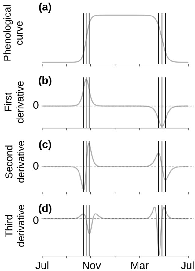
565 Figure 2: Schematic based off of Fig. 2 in Zhang et al. (2003) describing the selection of transition dates (shown using the vertical lines). (a) illustrates an example phenological curve of green-down and green-up. (b) illustrates the first derivative. (c) illustrates the second derivative where the root (second derivative equals 0) gives the value of the middle of season date. (d) illustrates the third derivative where the roots give the start and end of both seasons.
