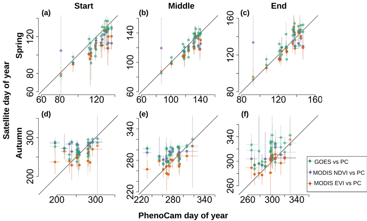
Figure 5: Scatter plots showing how the different data sources compare for their estimation of spring start (a), middle (b), and end (c); and autumn start (d), middle (e), and end (f). Median transition dates are indicated by the point and 95% credible intervals are indicated by the lines. The x -axis gives the day of year of the PhenoCam (PC) transition and the y -axis indicates the day of year of the different satellite data sources, which are color-coded as indicated in the legend. Spring correlations are much higher than autumn ones and GOES dates are more correlated at the start and middle of spring (a and b), but are slightly biased late at the end of spring (c).
