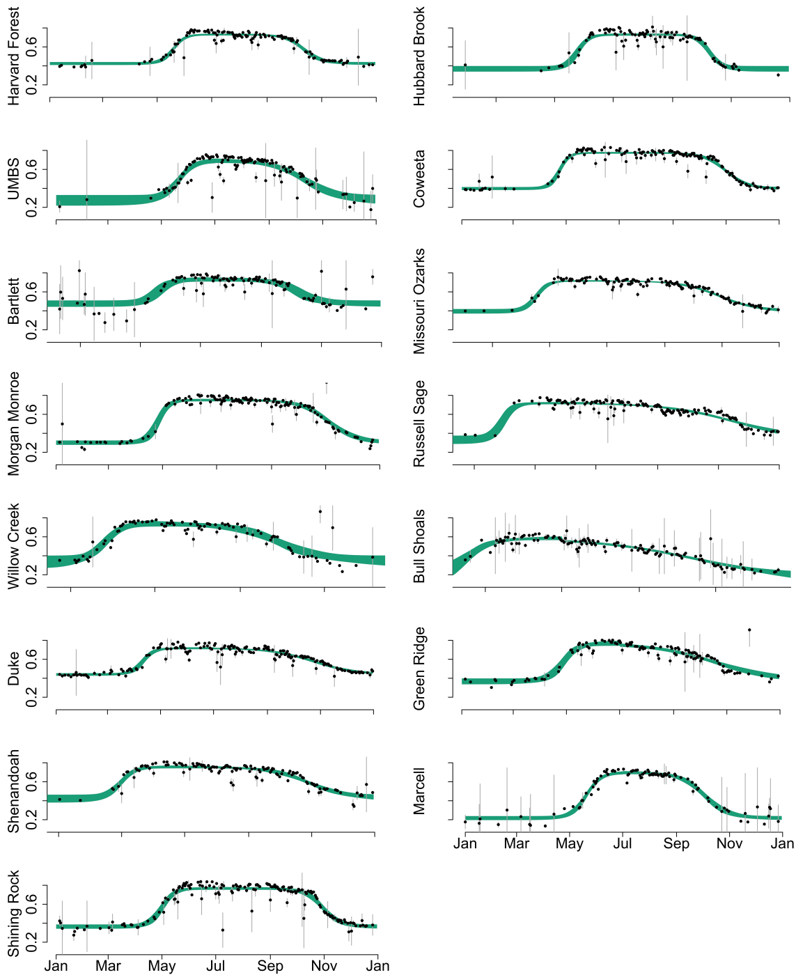
60 Figure S4: Phenological fits for GOES data at the different sites for 2019. The shading indicates the 95% credible intervals (CI). The points indicate the mean of the midday NDVI values from the daily diurnals with the gray vertical lines indicating the 95% CI on the daily data.
