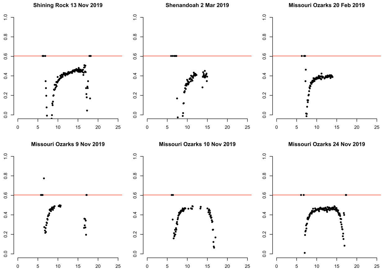
50 Figure S1: Examples of diurnal GOES data that show the consistent noisy NDVI value of 0.6040 (horizontal red line), which we removed to improve fits.
