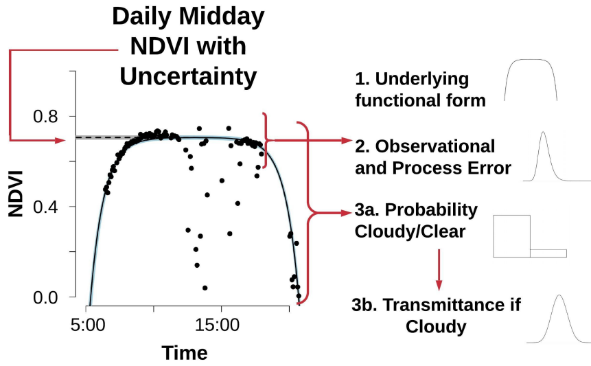
Figure S2: Representation of the GOES diurnal method used to estimate daily midday NDVI values. Reprinted from (Wheeler and Dietze, 2019).
