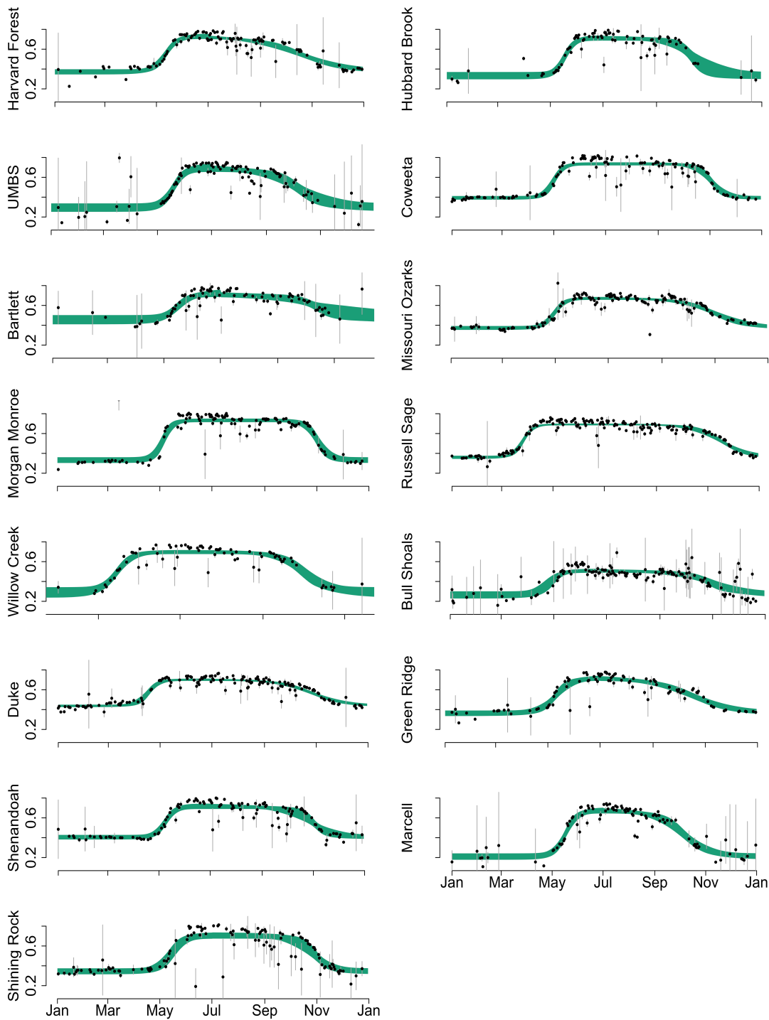
Figure S3: Phenological fits for GOES data at the different sites for 2018. The shading indicates the 95% credible intervals (CI). The points indicate the mean of the midday NDVI values from the daily diurnals with the gray vertical lines indicating the 95% CI on the daily data.
