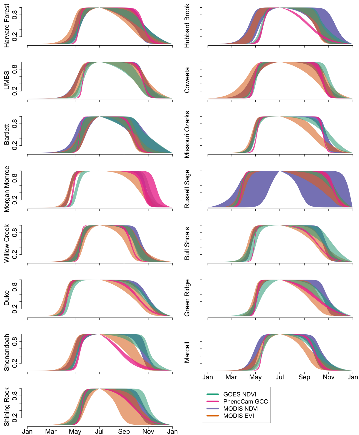
Figure S5: Rescaled 95% credible intervals for the phenology fits for 2018 for all data sources and sites.
