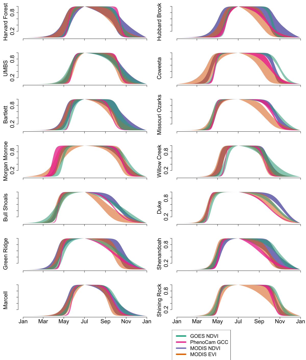
Figure S6: Rescaled 95% credible intervals for the phenology fits for 2019 for all data sources and sites.
