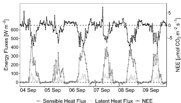
Figure 11. Energy and NEE fluxes from the Maritime Pine stands during a rainless period towards the end of the first post-fire hydrological year, from 04 to 09 September 2018.
