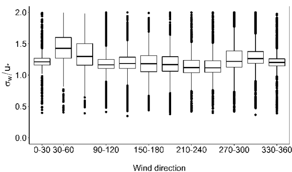
Figure 6. Box plots of the normalized standard deviation of the vertical wind velocity ( \sigma_w/u_* ) for the individual wind direction sectors.
