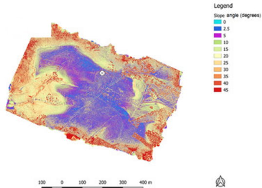
90 Figure 1. Slope angle map derived from aerial photography of the burnt area surrounding the flux tower. The imagery was acquired on 18 July 2028, using the standard RGB camera mounted on a DJI Phantom 3 drone.
