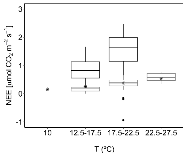
295 Figure 7. Box plots of the nighttime NEE fluxes for 5K temperature classes under soil moisture conditions that ranged from very dry to dry (VWC classes 1 and 2: grey boxes) and from intermediate to wet (VWC-classes 3 and 4: black boxes). The asterisks indicate the respiration fluxes calculated following the parameterization of the Lloyd-Taylor function.
