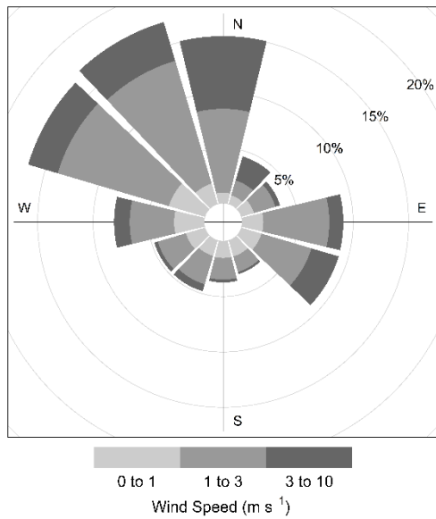
105 Figure 3. Wind rose of the study area over the first post-fire hydrological year (01 October 2017 – 30 September 2018), based on the sonic anemometer measurements at 11.6 m height.
