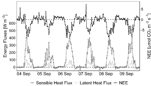
440 Figure 11. Energy and NEE fluxes from the Maritime Pine stands during a rainless period towards the end of the first post-fire hydrological year, from 04 to 09 September 2018.
