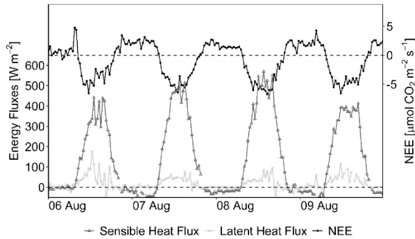
445 Figure 12. Daily cycles of 30-min sensible and latent heat fluxes and NEE fluxes during a rainless period in mid-summer, from 6 to 9 August 2018, when these fluxes originated from the eucalypt patches.
