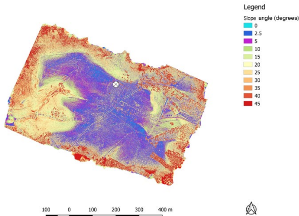
90 Figure 1. Slope angle map derived from aerial photography of the burnt area surrounding the flux tower. The imagery was acquired on 18 July 2018, using the standard RGB camera mounted on a DJI Phantom 3 drone.
