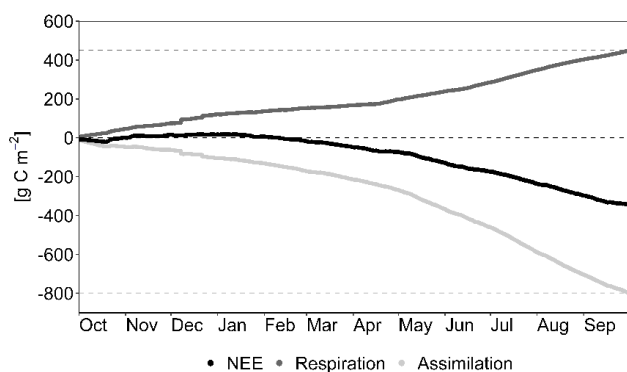
Figure 13. Cumulative NEE, assimilation and respiration fluxes during the first hydrological year after wildfire, from 01 October 2017 to 30 September 2018.
