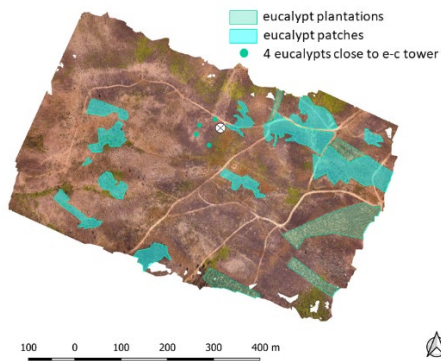
95 Figure 2. Ortho-photomap of the study area showing the Eucalypt stands as well as the 4 individual Eucalypt specimens close to the slim tower (circle with cross), the rest of the area consisting of Maritime Pine stands, The imagery was acquired on 18 July 2018, using a standard RGB camera mounted on a DJI Phantom 3 drone.
