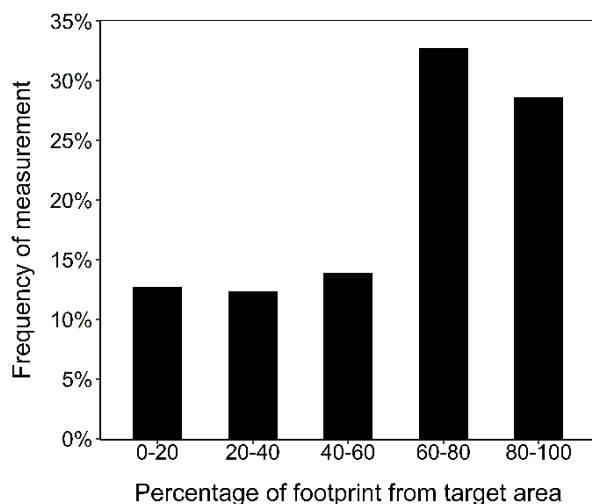
150 Figure 5. Distribution of the eddy covariance measurements during the first post-fire hydrological year over five classes of footprint area based on the degree of correspondence to the Maritime Pine stands.
