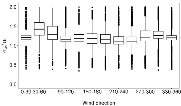
205 Figure 6. Box plots of the normalized standard deviation of the vertical wind velocity ( \sigma_w/u_* ) for the individual wind direction sectors.
