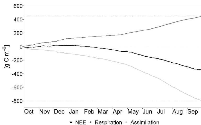
435 Figure 11. Cumulative NEE, assimilation and respiration fluxes during the first hydrological year after wildfire, from 01 October 2017 to 30 September 2018.
