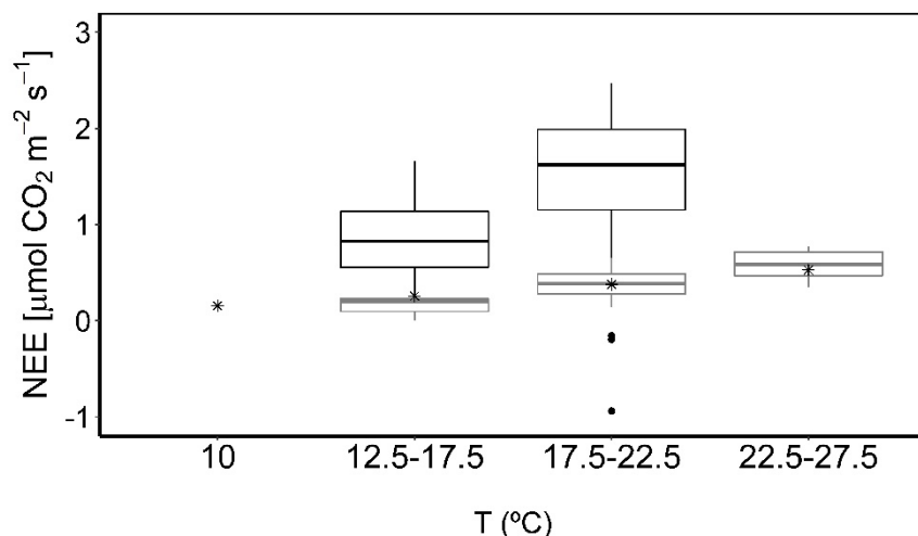
295 Figure 7. Box plots of the nighttime NEE fluxes for 5K temperature classes under very dry to dry (VWC classes 1 and 2: grey boxes) and intermediate to wet soil moisture conditions (VWC-classes 3 and 4: black boxes). The asterisks indicate the respiration fluxes calculated following the parameterization of the Lloyd-Taylor function.
