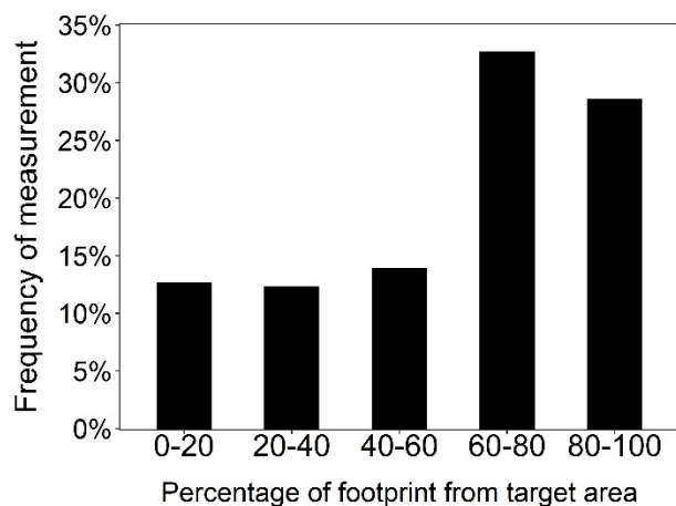
Figure 4. Distribution of the eddy covariance measurements during the first post-fire hydrological year over five classes of footprint area based on the degree of correspondence to the Maritime Pine stands
