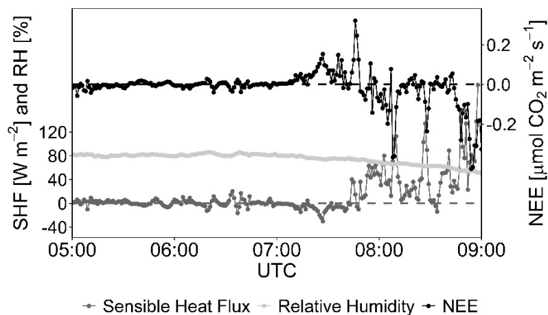
360 Figure 8. Relative humidity (RH) and sensible heat (SHF) and NEE fluxes with a 1-min resolution during the morning hours of 28 September 2017, indicating dew formation followed by evaporation of dew and associated CO 2 emission between 06:30 and 07:30 UTC.
