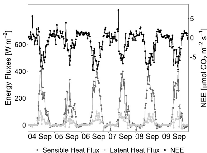
Figure 10. Energy and NEE fluxes from the Maritime Pine stands during a rainless period towards the end of the first post-fire hydrological year, from 04 to 09 September 2018.
