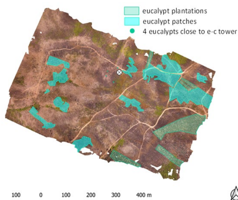
85 Figure 1. Ortho-photomap of the study area showing the Eucalypt stands as well as the 4 individual Eucalypt specimens close to the slim tower (cycle with cross), the rest of the area consisting of Maritime Pine stands
