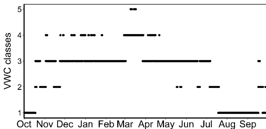
Figure 5. Volumetric water content (VWC) classes of the topsoil (from dry (1) to wet (5), as defined in Table 2) during the hydrological year 2017/18. The corresponding 30-minute VWC values are in Supplementary Figure S2.
