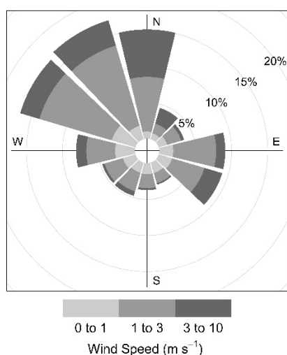
95 Figure 2. Wind rose of the study area over the first post-fire hydrological year (01 October 2017 – 30 September 2018), based on the sonic anemometer measurements at 11.6 m height.
