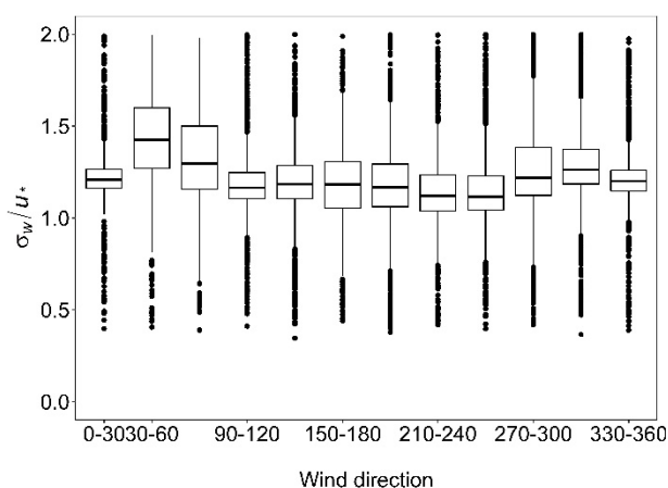
Figure 6. Box plots of the normalized standard deviation of the vertical wind velocity ( \sigma_w/u_* ) for the individual wind direction sectors.
