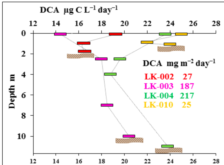
Fig. 4. Fig. 4. Dark \text{CO}_2 assimilation (DCA) in four lakes of the Yamal Peninsula (August 2019) in the water horizons, \mu\text{g C L}^{-1} \text{ day}^{-1} ; and integral PP for the entire water column, \text{mg C m}^{-2} \text{ day}^{-1} .
