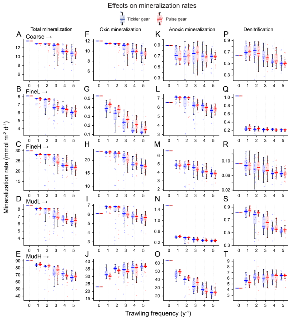
Figure 6: Rates of total mineralization (A - E), and the three main mineralization processes (F - J: oxic; K - O: anoxic; P - T: denitrification) ( \text{y} -axis, \text{mmol m}^{-2} \text{d}^{-1} ) for each gear type (blue boxes: tickler gear; red boxes: pulse gear), and for increasing trawling frequency ( \text{x} -axis, \text{y}^{-1} )
