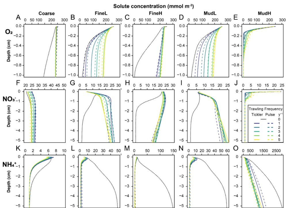
Figure 4: Annually averaged modelled concentrations ( mmol\ m^{-3} ) of oxygen (A - E), nitrate (F - J), and ammonium (K - O; rows) in the different types of sediment used as the basis for the disturbance simulations (columns). Black dotted line is the 0 trawl default, full and dotted coloured lines are tickler and pulse gear respectively, with increasing trawling frequencies as different colours.
