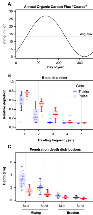
715 Figure 2: (A) Example of sinusoidal varying organic carbon deposition flux, based on average DIC efflux measured by Toussaint et al. (2020) for the Coarse sediment. (B) Simulated depletion of bioturbation, relative to the maximum (y-axis), with increasing trawling frequency ( \text{y}^{-1} , x-axis) in fine sands. Doy = day of year. (C) Imposed mixing and erosion depths (cm), for fine sandy and muddy sediments, for the two gear types (tickler chain and pulse gear).
