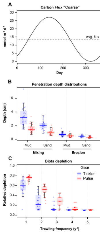
740 Figure 3: (A) Example of sinusoidal-varying carbon flux, based on average DIC efflux measured by Toussaint et al. (2020) for the Coarse sediment. (B) Imposed mixing and erosion depths (cm), for fine sandy and muddy sediments, for the two gear types (ticker chain and pulse gear). (C) Simulated depletion of bioturbation, relative to the maximum (y-axis), with increasing trawling frequency ( \text{y}^{-1} , x-axis) in fine sands. Day = day of year.
