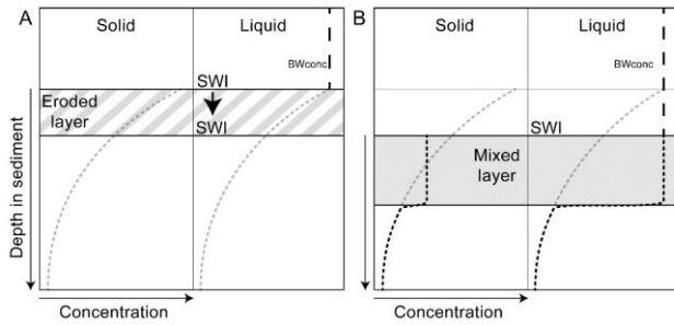
725 Figure 3: Implementation of a trawling event, on sediment concentrations of solids and liquids. Dotted grey lines: initial concentration profile, black line: profile after the event. (A) Hydraulic erosion removes a layer of sediment, moving the sediment-water interface (SWI) downward; the effect is implemented similarly for solids and liquids. (B) Subsequent mixing of the sediment homogenises the solid concentration over the mixed layer depth whereas liquids are set to the overlying bottom water concentration (BWconc). Depths of both impacts are defined in the text.
