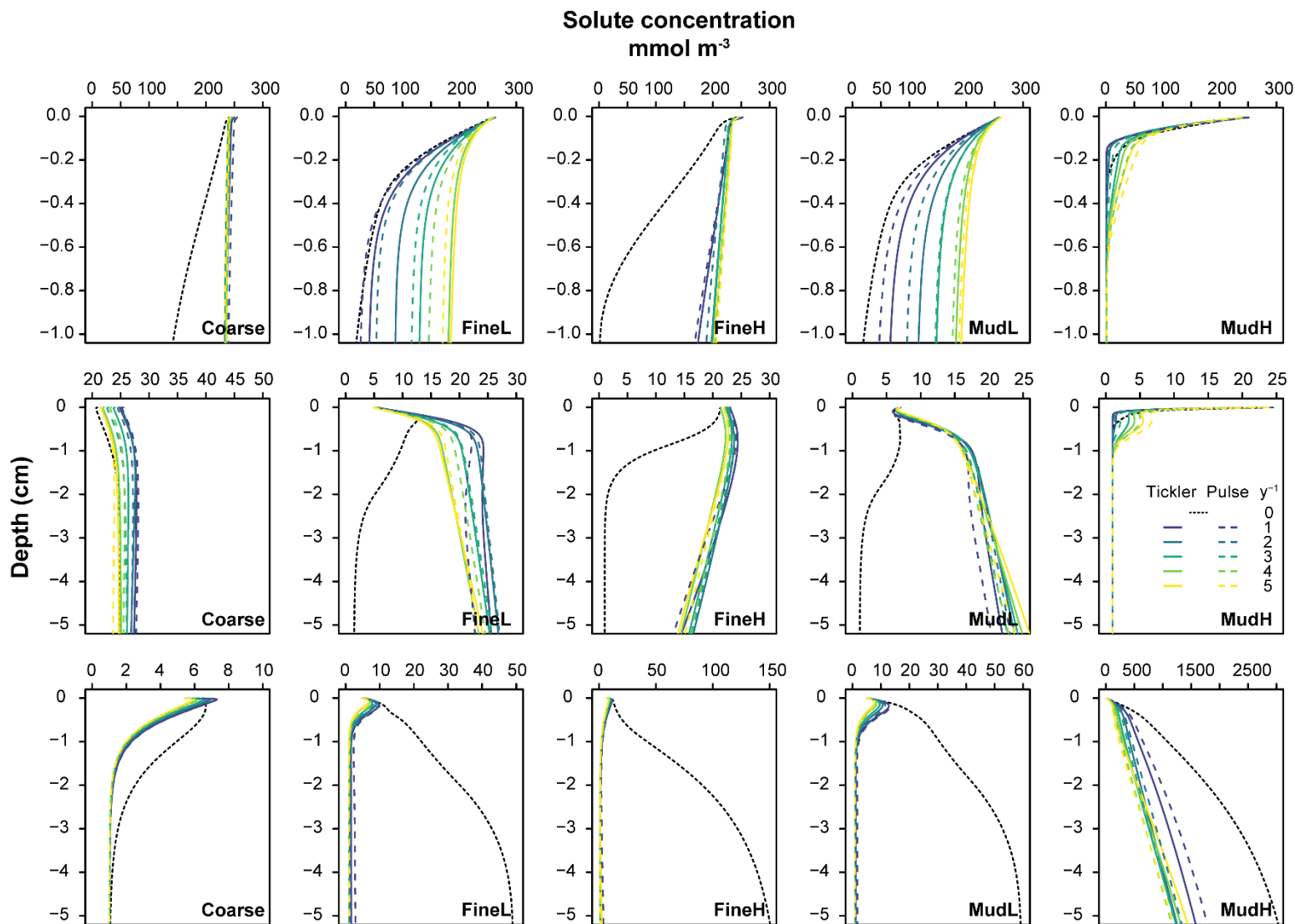
5 Figure S 2: Annually averaged modelled for oxygen, nitrate, and ammonium (mmol m -3 , rows) in the different types of sediment used as the basis for the disturbance simulations (columns). Black dotted line is the 0 trawl default, full and dotted coloured lines are tickler and pulse gear respectively, with increasing trawling frequencies as different colours.
