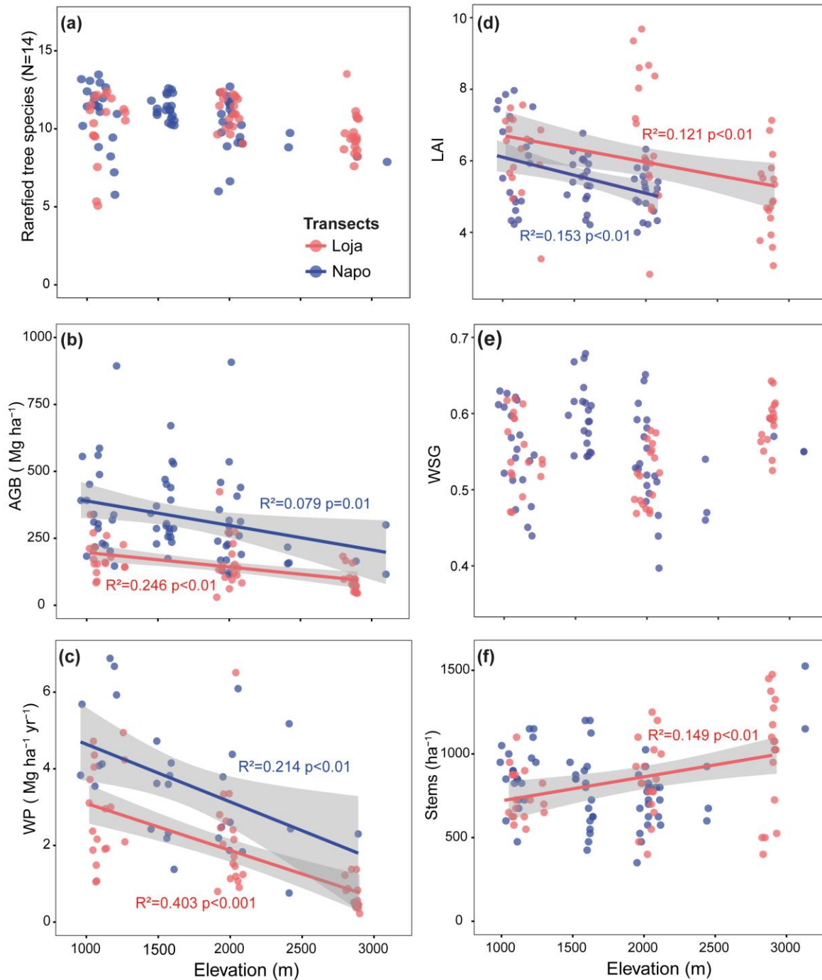
195 Figure 2. Variation of tree diversity (a), aboveground biomass (b), wood production (c), LAI (d), wood specific gravity (e), and stem density (f) along the two studied forest transects (red dots: Loja-transect, blue dots: Napo-transect). The number of plots available for a given parameter and transect varies, as not all parameters were measured in all plots (a: Loja 54 plots / Napo 64 plots; b: 54/66; c: 54/29; d: 53/60; e: 54/66; f: 54/66). Data presented in b, c, e and f were compiled from Unger et al. (2012), Leuschner et al. (2013), Kessler et al. (2014); data from the Napo transect in d are from Unger et al. (2013).
