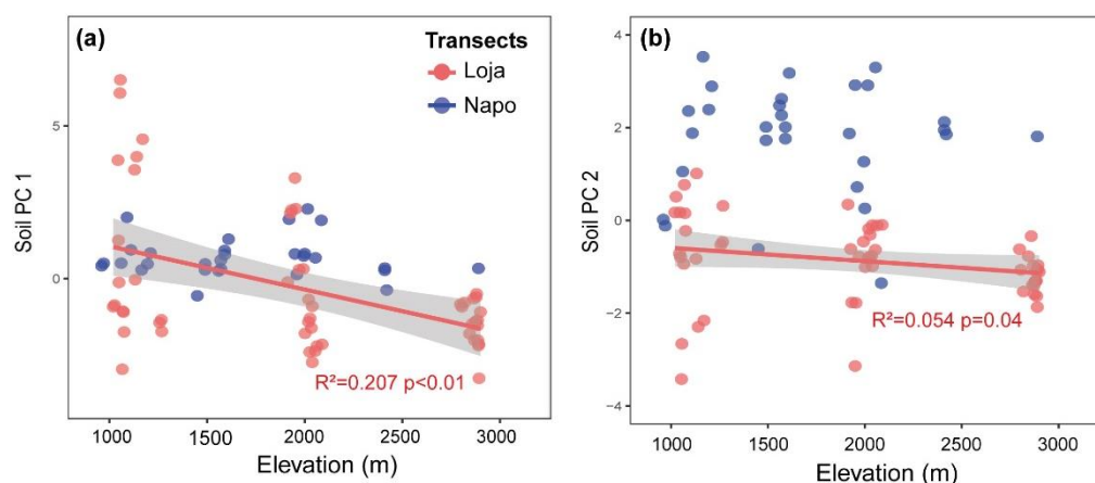
215 Figure 3. Variation of soil properties along the two forest transects (red dots: Loja-transect, blue dots: Napo-transect). Shown are the (a) first and (b) second principal components of the soil PCA (see Figure B1 and table B1).
