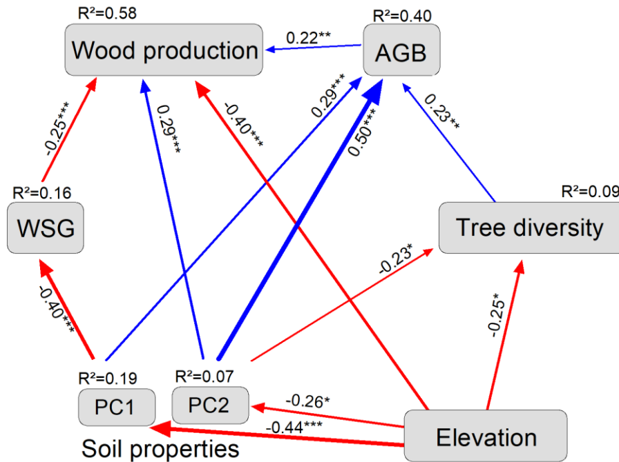
225 Figure 4. Final model for wood production (Loja-transect and Napo-transect: 83 plots). Structural equation model (chi-square = 8.4, 9 df, p = 0.50 , AIC 60.4, RMSEA < 0.01, CFI = 1.00) with standardized path coefficients. The size of the arrows is proportional to the strength of the paths, their significance is indicated by asterisks (* P < 0.05 , ** P < 0.01 , *** P < 0.001 ), blue arrows indicate positive and red negative estimates. AGB: aboveground biomass; WSG: wood specific gravity; PC1, PC2: first two axes of the soil PCA (Figure B1 and Table B1).
