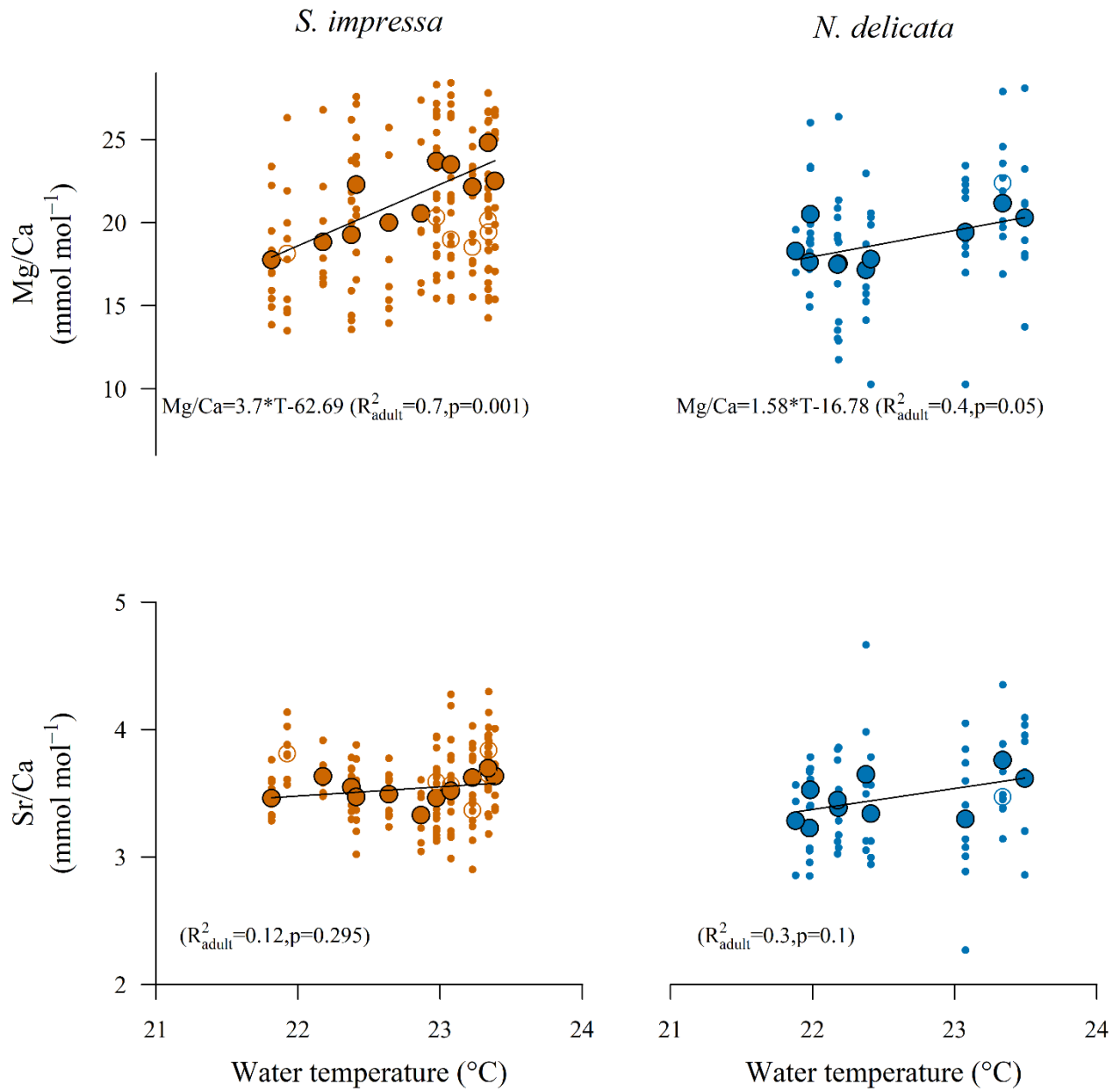
Figure 2 Relationships of Mg/Ca and Sr/Ca with annual temperature for adult (filled circles) and A-1 juvenile (open circles) ostracod samples of S. impressa ( \eta=7 ) and N. delicata ( \eta=3 ). Individual Single-shell samples are shown in light colors. Solid lines show the linear regressions for adult specimens.
