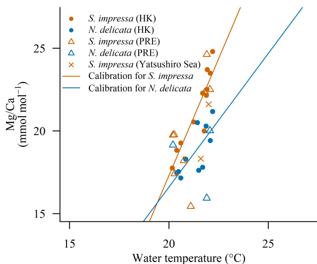
Figure 5. Mg/Ca ratios of ostracods from the PRE (OCEAN-HK) and Yatsushiro bay over the calibration for S. impressa ( \text{Mg/Ca}_{S. impressa} = 2.7 \cdot T - 37.2 ) and N. delicata ( \text{Mg/Ca}_{N. delicata} = 1.6 \cdot T - 15.7 ) performed with samples from Hong Kong (EPD). The BWT from the Copernicus product was used for OCEAN-HK samples. Surface water temperature from the Tanoura buoy in the last 15 d in June (21.8 °C) and November (21.9 °C) were considered for the Yatsushiro Sea samples.
