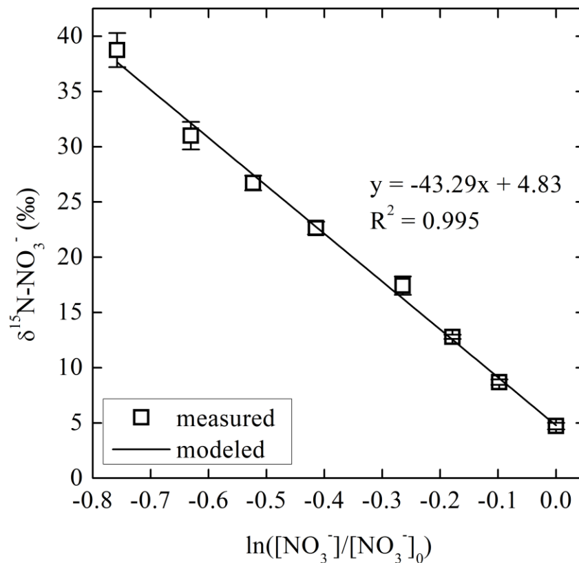
Figure S3. Rayleigh plot of \delta^{15}\text{N-NO}_3^- versus the natural logarithm of fractional \text{NO}_3^- consumption. The slope of linear regression gives an estimate of the apparent N isotope effect for \text{NO}_3^- consumption during the anoxic incubation.
