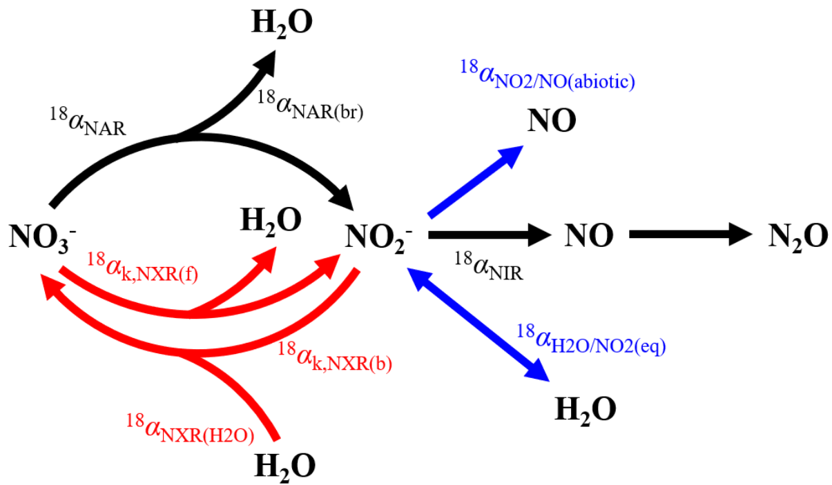
Figure S1. Model structure of co-occurring denitrification and \text{NO}_2^- re-oxidation and associated O isotopic fractionations. Values of the O isotopic fractionation factors are given in Table S3.
