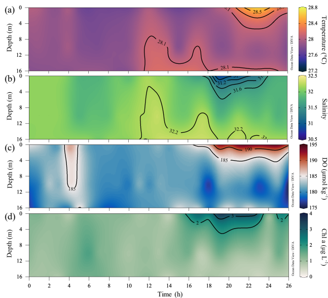
Figure 3: Time-series observations of (a) temperature (°C), (b) salinity, (c) DO ( \mu\text{mol kg}^{-1} ) and (d) Chl a concentrations ( \mu\text{g L}^{-1} ) at Station F303 (see Fig. 1b) from July 19-20, 2018 after the typhoon passage, showing the complete destruction and the subsequent rapid development of stratification.
