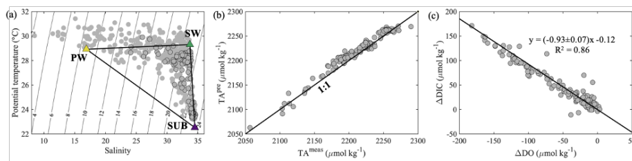
Figure 2: (a) Potential temperature ( ^{\circ}\text{C} ) vs. salinity, (b) predicted TA ( TA^{pre} , \mu\text{mol kg}^{-1} ) vs. measured TA ( TA^{meas} , \mu\text{mol kg}^{-1} ), and (c) \Delta DIC ( \mu\text{mol kg}^{-1} ) vs. \Delta DO ( \mu\text{mol kg}^{-1} ) on the NSCS shelf off the PRE. The black-edged circles represent bottom water samples with depths > 10 m. The yellow, green and purple triangles in (a) represent the endmember values of brackish plume water (PW), offshore surface water (SW) and upwelled subsurface water (SUB), respectively. The black line in (c) denotes the slope of \Delta DIC plotted against \Delta DO derived from the Model II regression.
