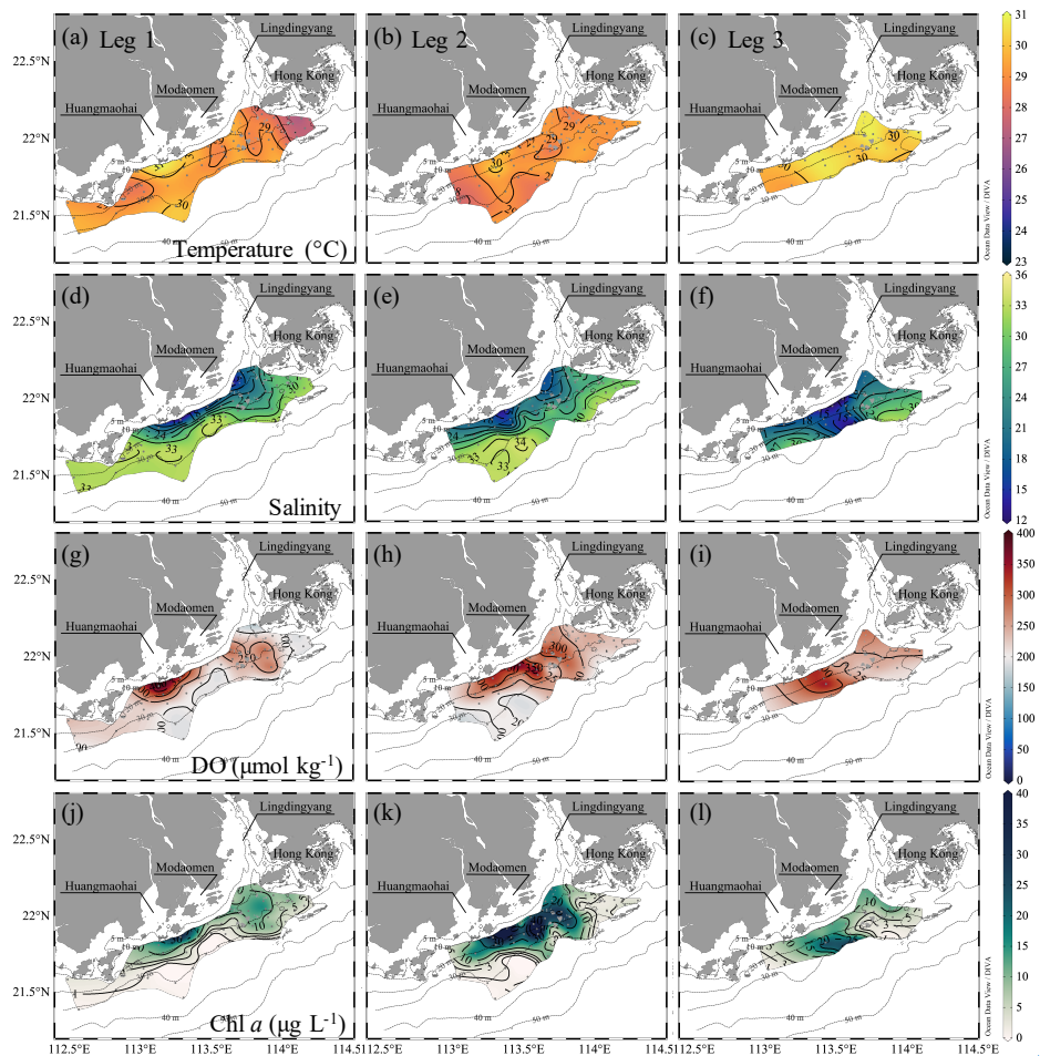
480 Figure 3: Distributions of temperature ( ^{\circ}\text{C} ), salinity, DO ( \mu\text{mol kg}^{-1} ) and Chl a concentrations ( \mu\text{g L}^{-1} ) at the surface water layer off the PRE during Leg 1 pre-typhoon, and during Legs 2 and 3 post-typhoon. The white and magenta contours in (g) and (w) show the hypoxic ( \text{DO} < 63 \mu\text{mol kg}^{-1} ) and oxygen-deficit ( \text{DO} < 94 \mu\text{mol kg}^{-1} ) zones. Figures were produced using Ocean Data View v. 5.3.0 ( http://odv.awi.de , last access: 08 June 2020).
