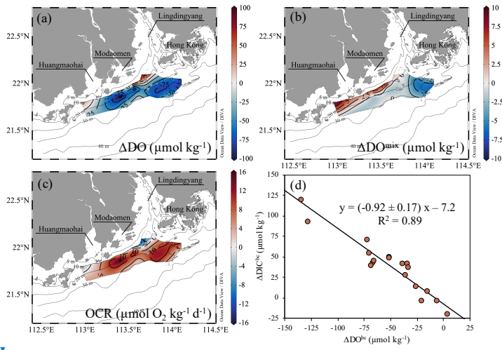
Figure 8: Distributions of (a) total DO changes ( \Delta DO , \mu\text{mol kg}^{-1} ), (b) mixing-induced DO changes ( \Delta DO^{\text{mix}} , \mu\text{mol kg}^{-1} ) and (c) the biochemical-induced oxygen consumption rate (OCR, \mu\text{mol O}_2 \text{ kg}^{-1} \text{ d}^{-1} ) between Leg 3 and Leg 2 on the inner NSCS shelf off the PRE. (d) The biochemical-induced changes in DIC ( \Delta \text{DIC}^{\text{bc}} , \mu\text{mol kg}^{-1} ) vs. DO ( \Delta \text{DO}^{\text{bc}} , \mu\text{mol kg}^{-1} ) in bottom waters with depths > 10 m from Leg 2 to Leg 3. The black line denotes the slope of \Delta \text{DIC}^{\text{bc}} plotted against \Delta \text{DO}^{\text{bc}} derived from the Model II regression.
