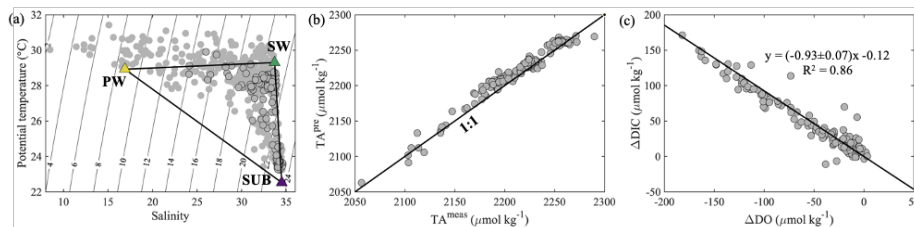
185 Figure 2: (a) Potential temperature ( ^{\circ}\text{C} ) vs. salinity, (b) predicted TA ( TA^{pre} , \mu\text{mol kg}^{-1} ) vs. measured TA ( TA^{meas} , \mu\text{mol kg}^{-1} ), and (c) \Delta DIC ( \mu\text{mol kg}^{-1} ) vs. \Delta DO ( \mu\text{mol kg}^{-1} ) on the NSCS shelf off the PRE. The black-edged circles represent bottom water samples with depths > 10 m. The yellow, green and purple triangles in (a) represent the endmember values of brackish plume water (PW), offshore surface water (SW) and upwelled subsurface water (SUB), respectively. The black line in (c) denotes the slope of \Delta DIC plotted against \Delta DO derived from the 190 Model II regression.
