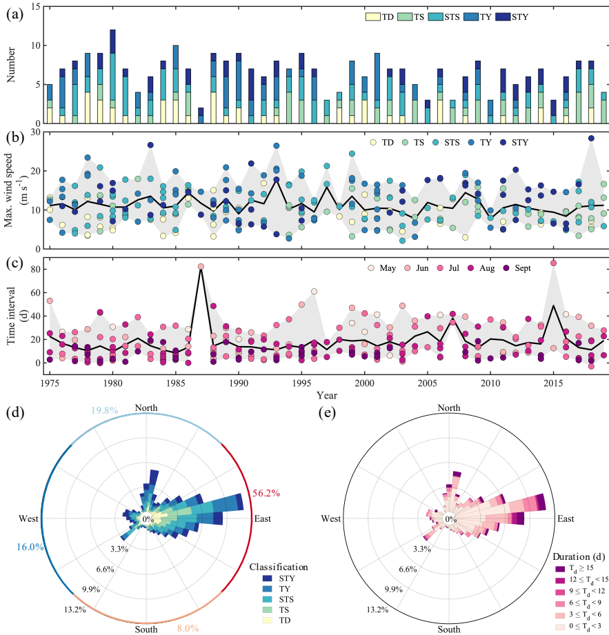
545 Figure 9: Statistics of tropical cyclones passing the northern South China Sea (NSCS) from May to September over 1975-2019. (a) Numbers of tropical cyclones. TD, TS, STS, TY and STY represent tropical depressions (the maximum wind speed near the centre is between 10.8-17.1 m s^{-1} over its lifetime), tropical storms (17.2-24.4 m s^{-1} ), strong tropical storms (24.5-32.6 m s^{-1} ), typhoons (32.7-41.4 m s^{-1} ) and strong typhoons (41.5-50.9 m s^{-1} ), respectively. (b) The maximum wind speed of each tropical cyclone. The black line and grey shadow denote the annual average and range of the maximum wind speeds. (c) The time interval between two successive tropical cyclones. The black line and grey shadow denote the annual average and range of the time intervals. The negative time interval indicates an overlap in time of two
