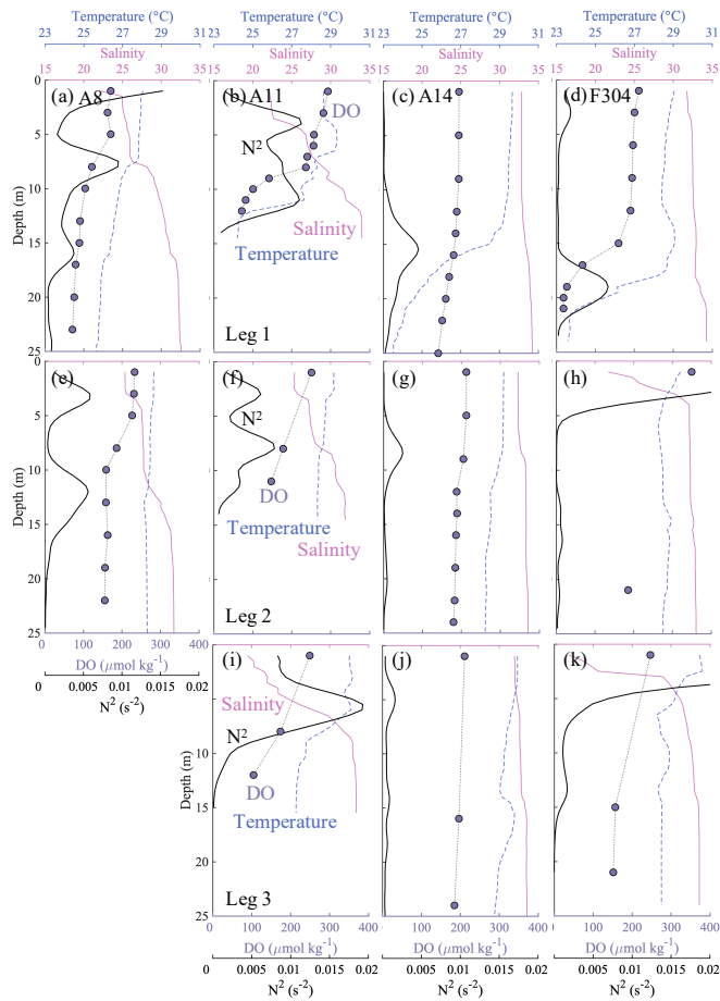
Figure 7: Profiles of temperature (°C) (blue dashed lines), salinity (pink solid lines), dissolved oxygen (DO, μmol kg -1 ) (purple dots) and buoyancy frequency N^2 (s -2 ) (bold black solid lines) at stations A8, A11, A14 and F304 (see Fig. 1b), with visits both pre-typhoon (Leg 1) and post-typhoon (Legs 2 and 3). The vertical distributions of N^2 have been smoothed by the Gaussian method.
