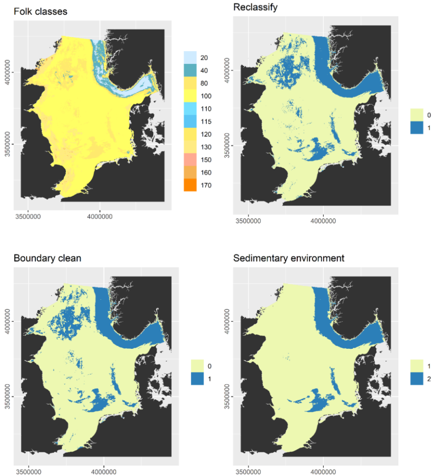
860 865 Figure A1: Derivation of the sedimentary environment layer: Folk textural classes were derived from sediment composition predicted by Mitchell et al. (2019). 20 – Mud, 40 – Sandy mud, 80 – Muddy sand, 100 – Sand, 110 – Gravelly mud, 115 – Gravelly sandy mud, 120 – Gravelly muddy sand, 130 – Gravelly sand, 150 – Muddy sandy gravel, 160 – Sandy gravel, 170 – Gravel. Mud, sandy mud, and muddy sand were reclassified as potential accumulation (1), the remainder as erosion/non-deposition (0) areas. The polygons were simplified with the Boundary Clean tool in ArcGIS. The potential accumulation areas were critically reviewed in the light of measured sedimentation rates and geological interpretations of sediment cores (de Haas et al., 1997 and references therein) and the dominant areas of erosion/net-deposition (1) and sediment accumulation (2) derived.
