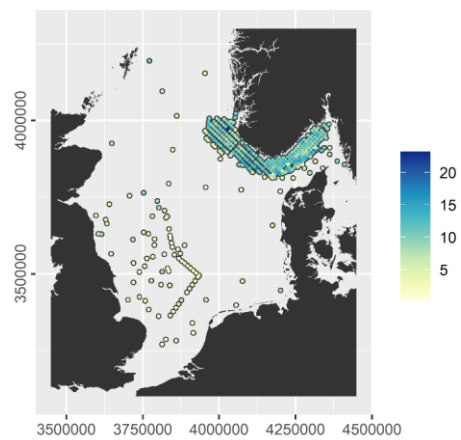
Organic Carbon Density ( \text{kg m}^{-3} )
