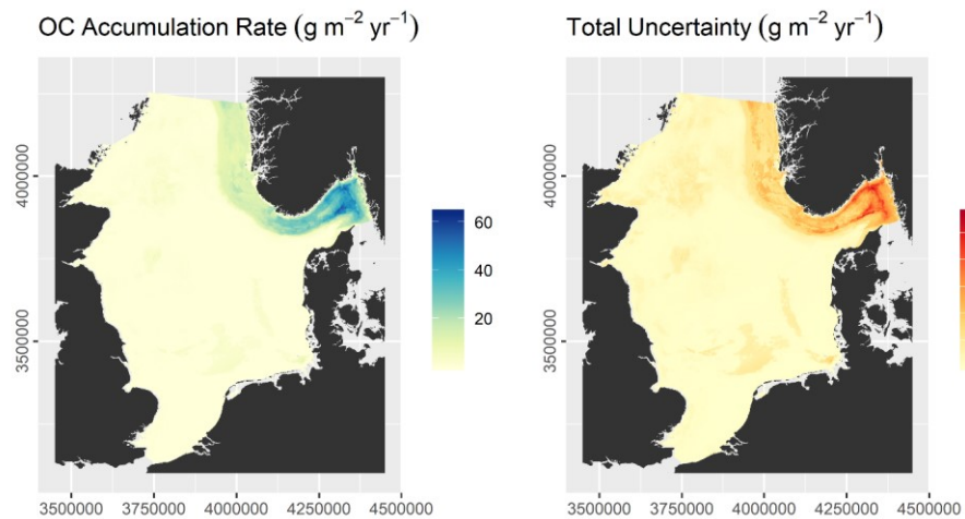
Figure 6: Calculated OC accumulation rate (left) and associated uncertainty (right)
