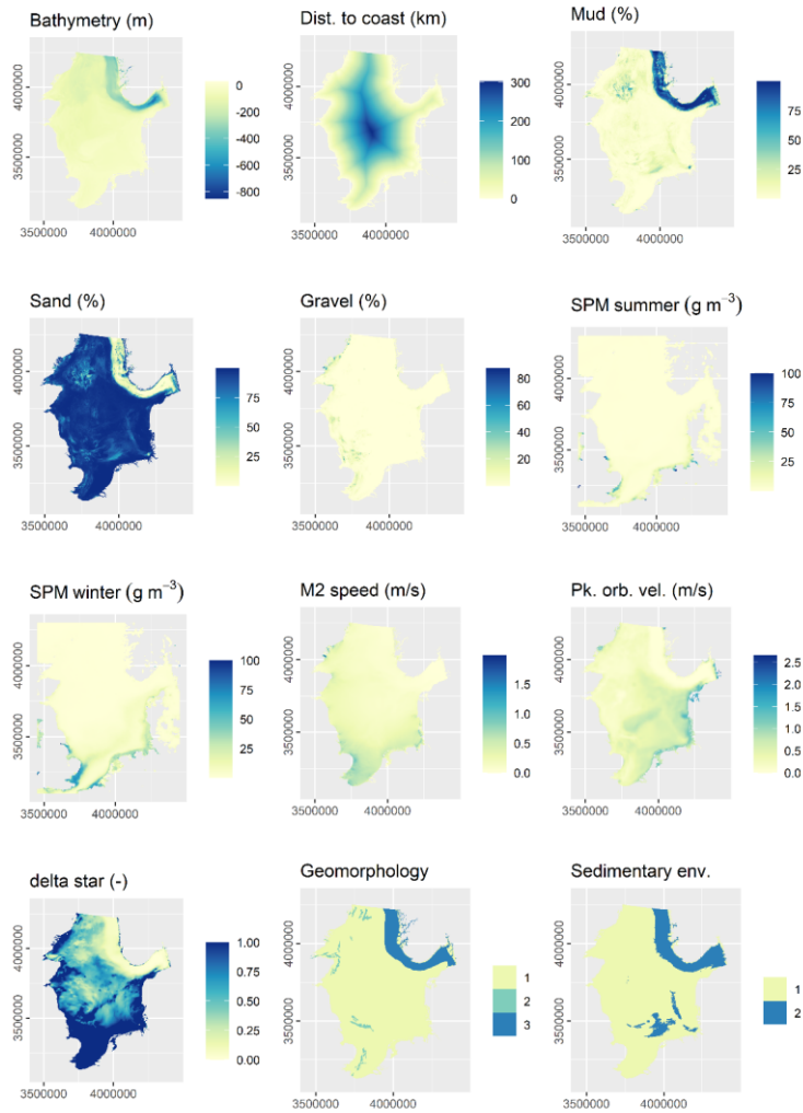
870 Figure A2: Selected predictor variables of the sedimentation rate model. Geomorphology: 1 - Shelf, 2 – Shelf valley, 3 – Glacial trough. Sedimentary environment: 1 – Erosion/non-deposition, 2 - Accumulation.
