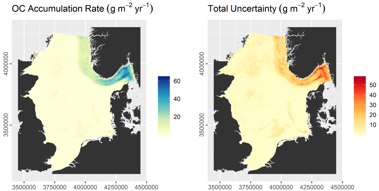
Figure 6: Calculated OC accumulation rate (left) and associated uncertainty (right)
