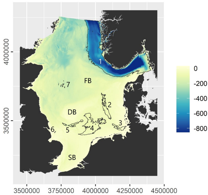
830 Figure 1: Overview of the study site. Letters refer to localities: DB – Dogger Bank; FB – Fisher Bank; SB – Southern Bight. Numbers refer to areas of sediment deposition: 1 – Norwegian Trough; 2 – Elbe palaeo-valley; 3 – German Bight; 4 – Oyster Ground; 5 – Outer Silver Pit; 6 – Inner Silver Pit; 7 – Devil’s Hole. Refer to chapter 3.2 for the delineation of areas of sediment deposition.
