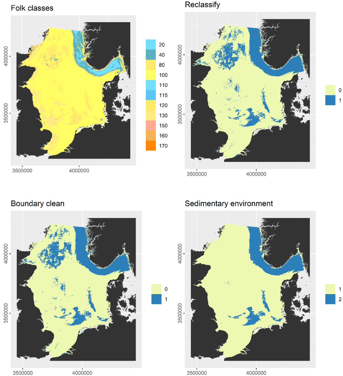
855 Figure A1: Derivation of the sedimentary environment layer: Folk textural classes were derived from sediment composition predicted by Mitchell et al. (2019). 20 – Mud, 40 – Sandy mud, 80 – Muddy sand, 100 – Sand, 110 – Gravelly mud, 115 – Gravelly sandy mud, 120 – Gravelly muddy sand, 130 – Gravelly sand, 150 – Muddy sandy gravel, 160 – Sandy gravel, 170 – Gravel. Mud, sandy mud, and muddy sand were reclassified as potential accumulation (1), the remainder as erosion/non-deposition (0) areas. 860 The polygons were simplified with the Boundary Clean tool in ArcGIS. The potential accumulation areas were critically reviewed in the light of measured sedimentation rates and geological interpretations of sediment cores (de Haas et al., 1997 and references therein) and the dominant areas of erosion/net-deposition (1) and sediment accumulation (2) derived.
