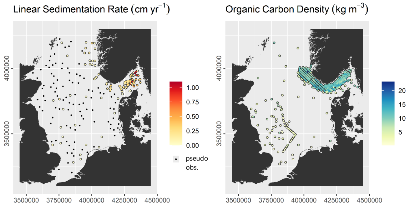
835 Figure 2: Available samples on sedimentation rate (left) and OC density (right)
