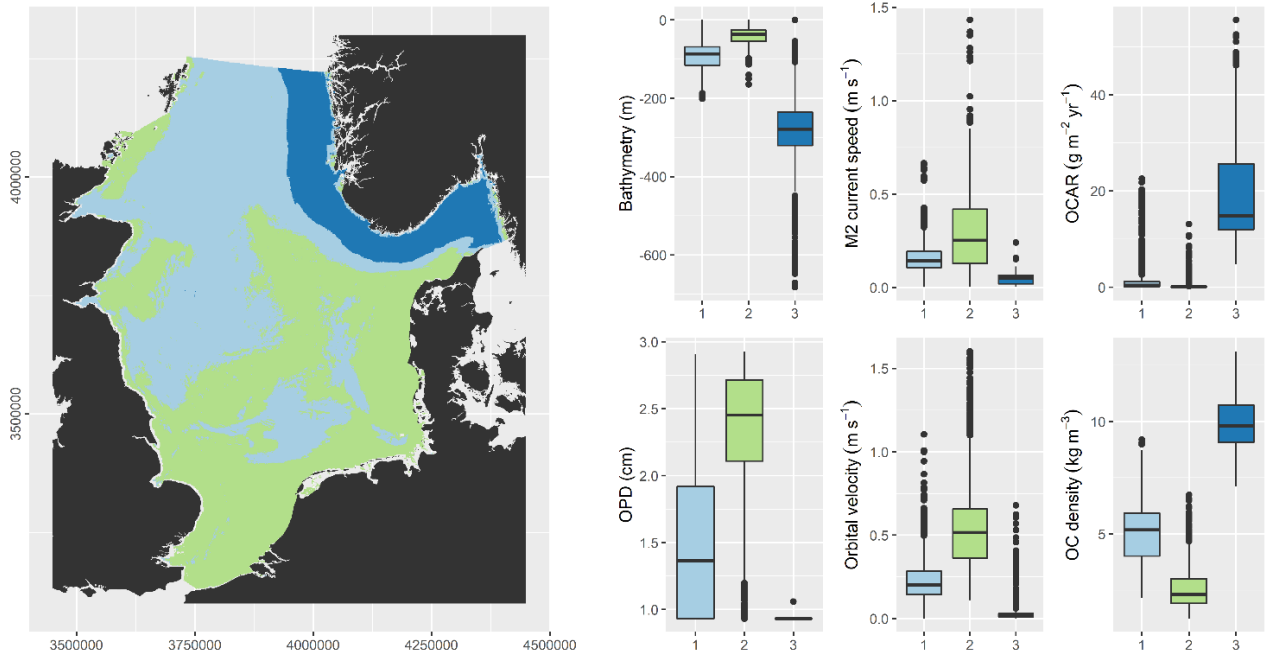
Figure 7: Regionalisation of the North Sea and Skagerrak: Region 1 (light blue) – transition zone; Region 2 (green) – turnover zone; Region 3 (dark blue) – burial zone. Note that boxplots are based on 10000 randomly placed points, rather than all pixels.
