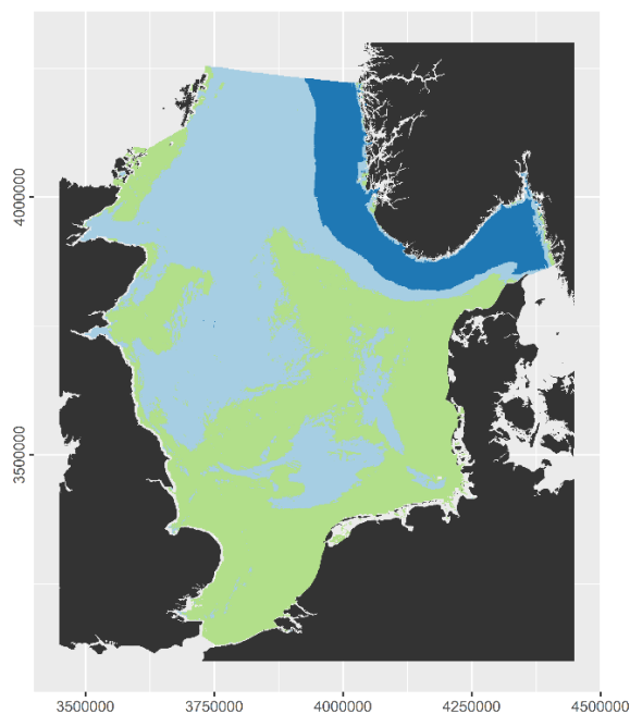
Figure 7: Regionalisation of the North Sea and Skagerrak: Region 1 (light blue) – transition zone; Region 2 (green) – turnover zone; Region 3 (dark blue) – burial zone. Note that boxplots are based on 10000 randomly placed points, rather than all pixels.
