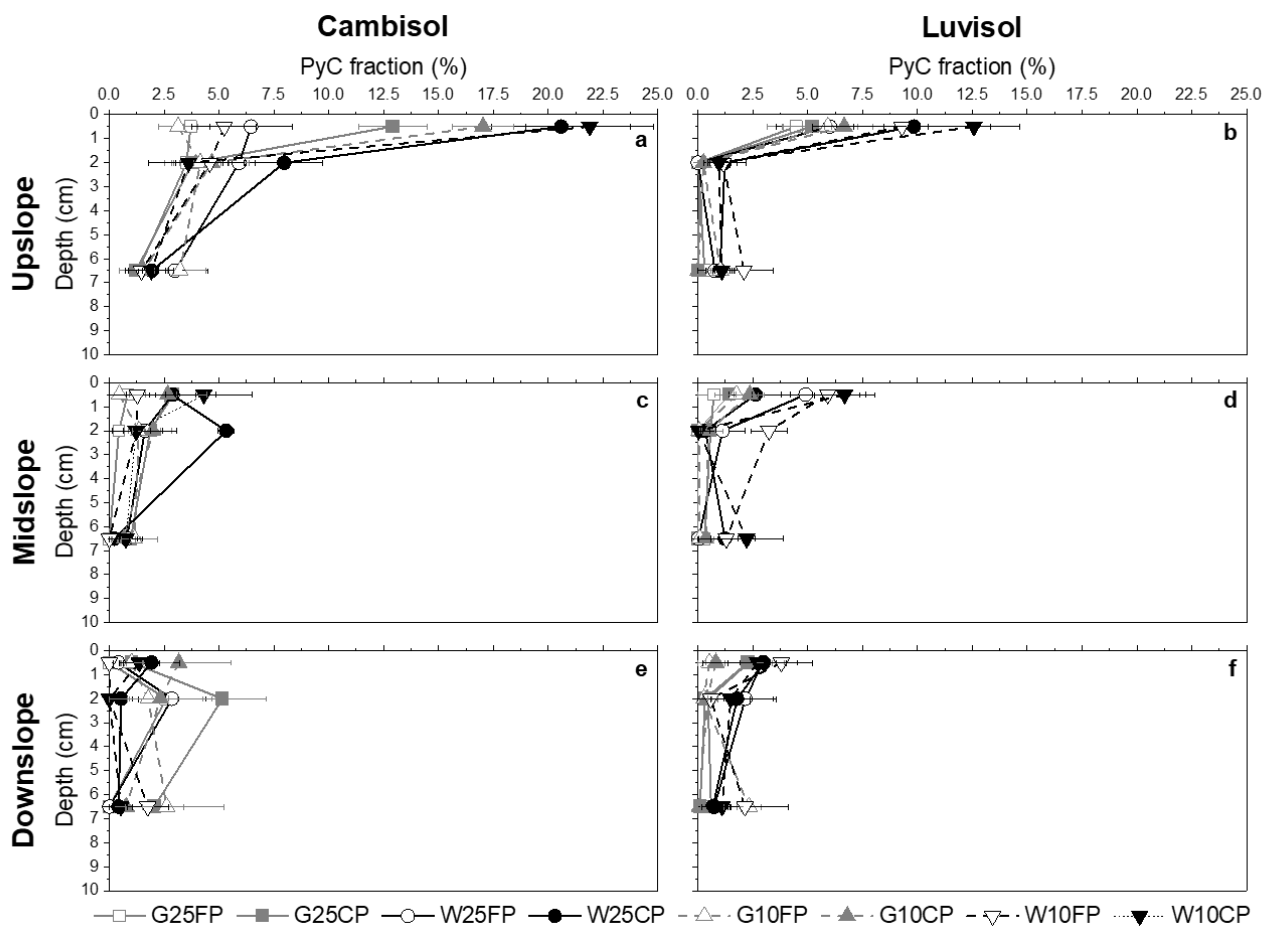
Figure 7: Distribution of PyC [PyC fraction = fraction of OC derived from the PyC in %] in soil cores for the Cambisol (a, c and e) and Luvisol (b, d and f) along the 0.25-m 2 plot (Upslope: a-b; midslope: c-d and downslope: e-f) and with depth (0-1, 1-3, 3-10 cm) for each treatment after 30 minutes rainfall (total: 51.4 ± 1.4 mm) (G = grass-PyC; W = wood-PyC; 25 = 25° slope; 10 = 10° slope; FP = fine PyC (< 63 µm); CP = coarse PyC (63 µm to 2 mm)). Average values ± 1 standard error (n=3).
