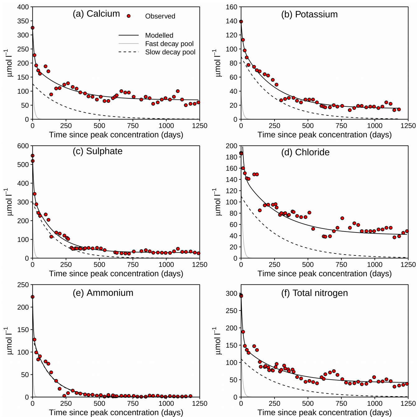
Figure 5: Fitted decay curves for solutes exhibiting a single concentration peak after the fire, Gärslöbäcken. See Table 3 for statistics and model fits for the other catchments.
