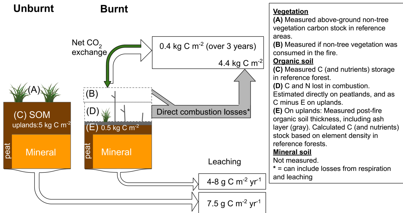
Figure 6: Conceptual C flow diagram during the first 3 years after the fire in a boreal forest catchment. Post-fire leaching is given as a range for the first three years, and leaching from an unburned catchment (Gärsjöbäcken, Table 2) is the mean of the four years before the fire occurred.
