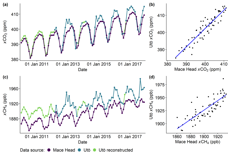
Figure A2. Monthly means of atmospheric (a) \text{CO}_2 and (c) \text{CH}_4 mole fractions from 2010 to 2017. We preferred data from Utö station (Finnish Meteorological Institute, Helsinki), which start in March 2012, due to their proximity to observations from SOOP Finnmaid . Concerning measurements on Utö, the method described in Kilkki et al. (2015) is applicable for the study period except that the Nafion dryer has not been in use since November 2013 (Juha Hatakka, pers. comm.). For the period before 2012 and to fill data gaps in September 2013 and 2016 in the Utö series, we used atmospheric data from Mace Head station (National University of Ireland, Galway) via the NOAA ESRL Carbon Cycle Cooperative Global Air Sampling Network (Dlugokencky et al., 2019a, b), which is roughly at similar latitude. To correct differences between both stations, we normalised the data from Mace Head to those from Utö based on the shared period from 2012 to 2017 using linear regression (b,d). This very simple approach is sufficient to evaluate the magnitude of super- and undersaturation and compare it on interannual scales.
