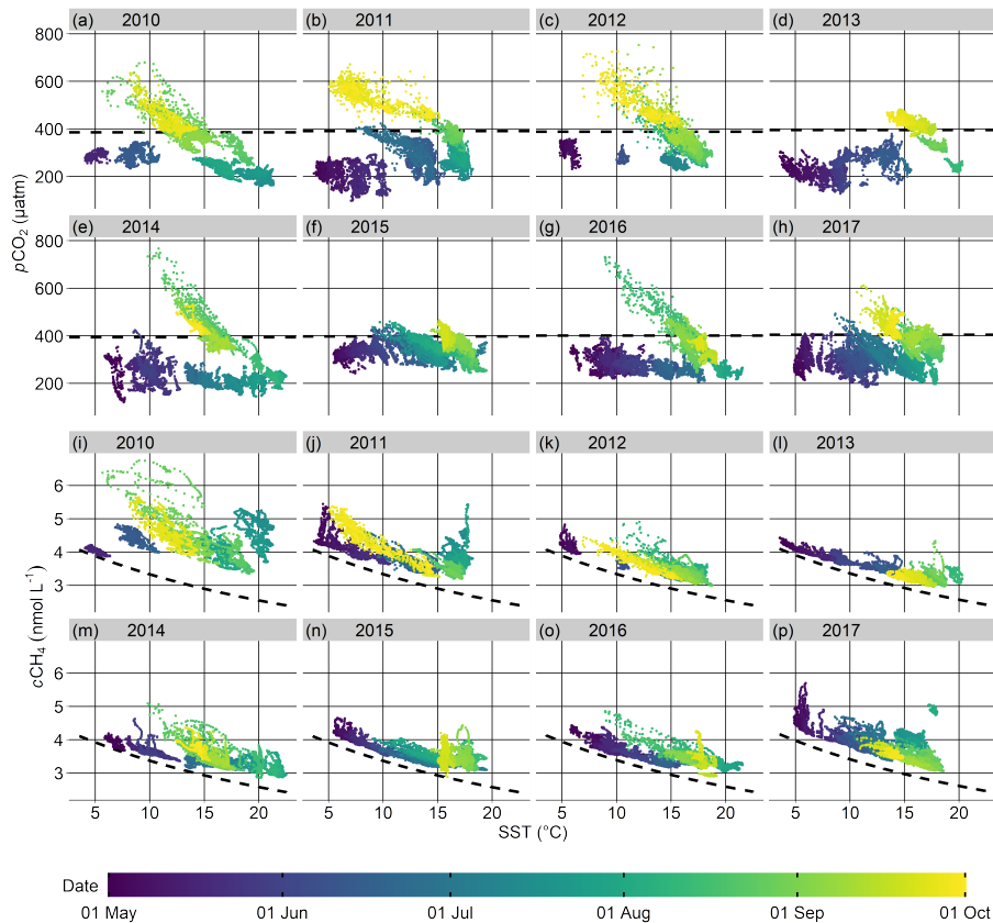
Figure 9. Surface \text{CO}_2 partial pressure (a–h), and \text{CH}_4 concentration (i–p) from 1 May to 30 September within box Ö-S, each plotted against temperature for individual years. The measurement date is colour-coded. Black dashed lines indicate atmospheric equilibrium partial pressure and concentration (calculated using mean seasonal salinity), respectively.
