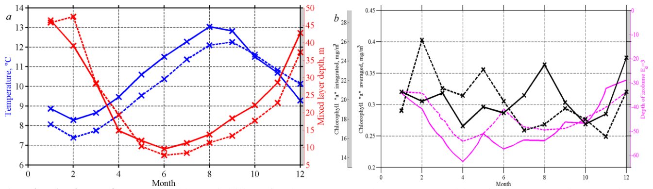
(Revised) Figure 3: a – Monthly variability of column-averaged temperature (blue) in the 0-70 m layer and mixed layer depth (red); b – Monthly variability of integral and column-averaged Chl in the 0-70 m layer (black color) and depth of isolume E_d=3 \mu\text{mol photons m}^{-2} \text{s}^{-1} (purple color) in 2016 (solid lines) and 2017 (dashed lines).
