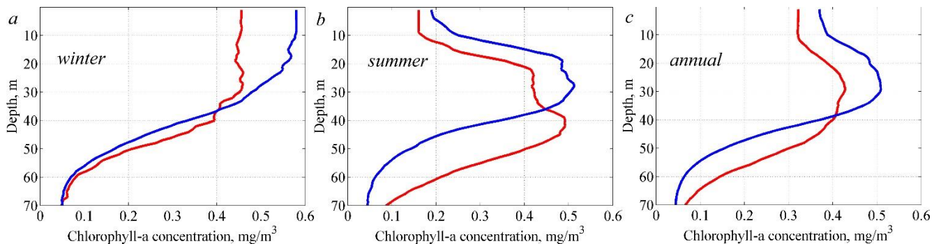
Figure 8: Average profile of Chl in 2016 (red line) and 2017 (blue line) in winter (January-March) (a), summer (June-August) (b) and annually-averaged (c).
