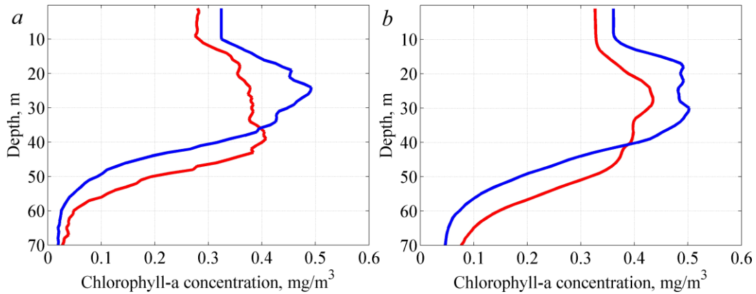
Supplementary Figure S2: Average profile of Chl in 2016 and 2017 by the measurements of the float #7900591 (a) and float #6901866 (b).
