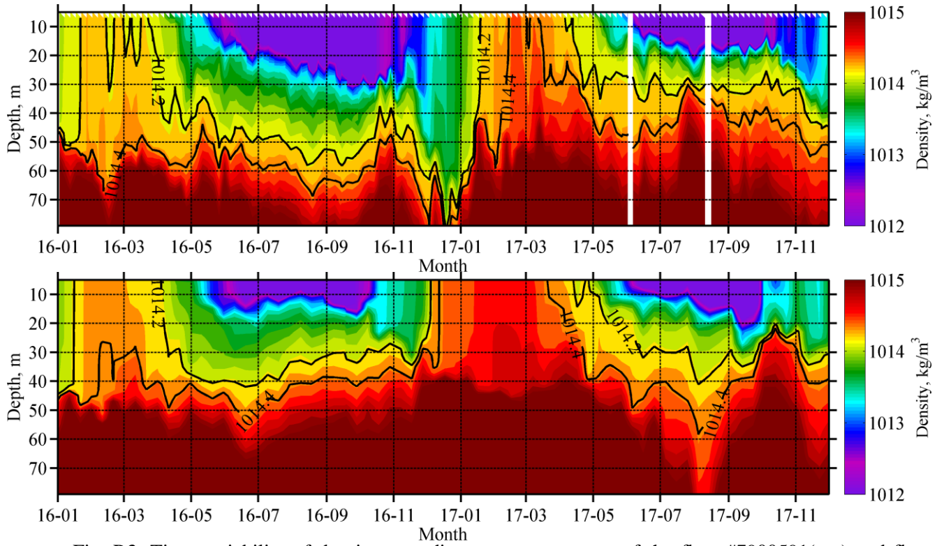
Fig. R3. Time variability of density according to measurements of the float #7900591(top) and float #6901866 (bottom)
