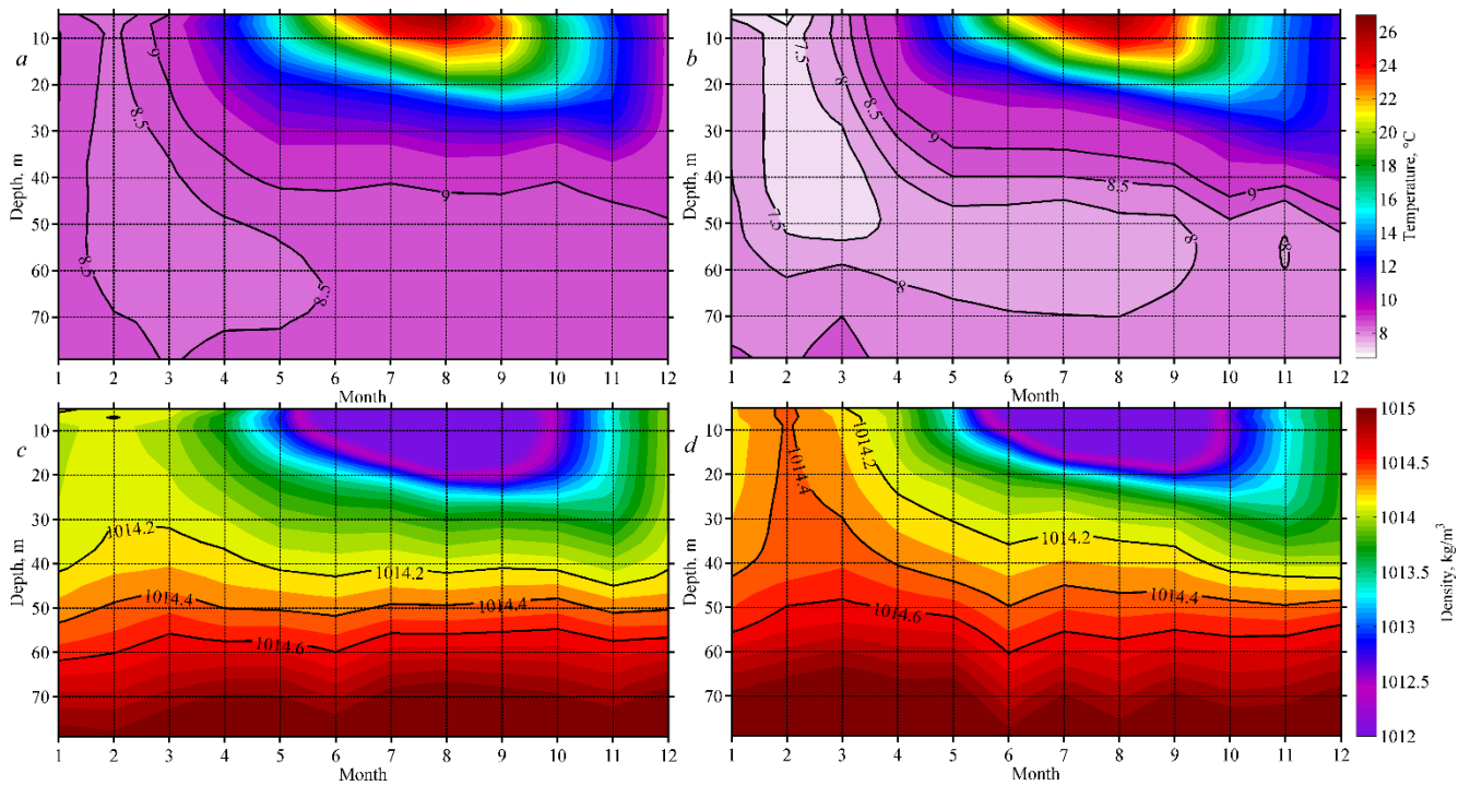
(Revised) Figure 2: Monthly vertical diagram of temperature in 2016 (a) and 2017 (b), potential density in 2016 (c) and 2017 (d).
