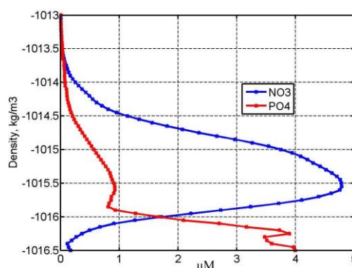
Fig. R1. Multiannual-averaged profile of nitrates (blue) and phosphates (red) in the central part of the Black Sea in \sigma -coordinates
