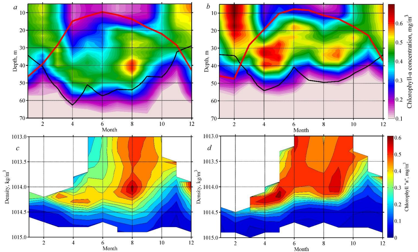
(Revised) Figure 4: Seasonal variability of Chl in 2016 ( a, c ) and 2017 ( b, d ) in z-coordinates (top panel) and density coordinates (bottom panel). The black line marks the border of the photic zone (maximum photosynthetic active radiation E_d=3 \mu\text{mol photons m}^{-2} \text{s}^{-1} ), the red line marks MLD.
