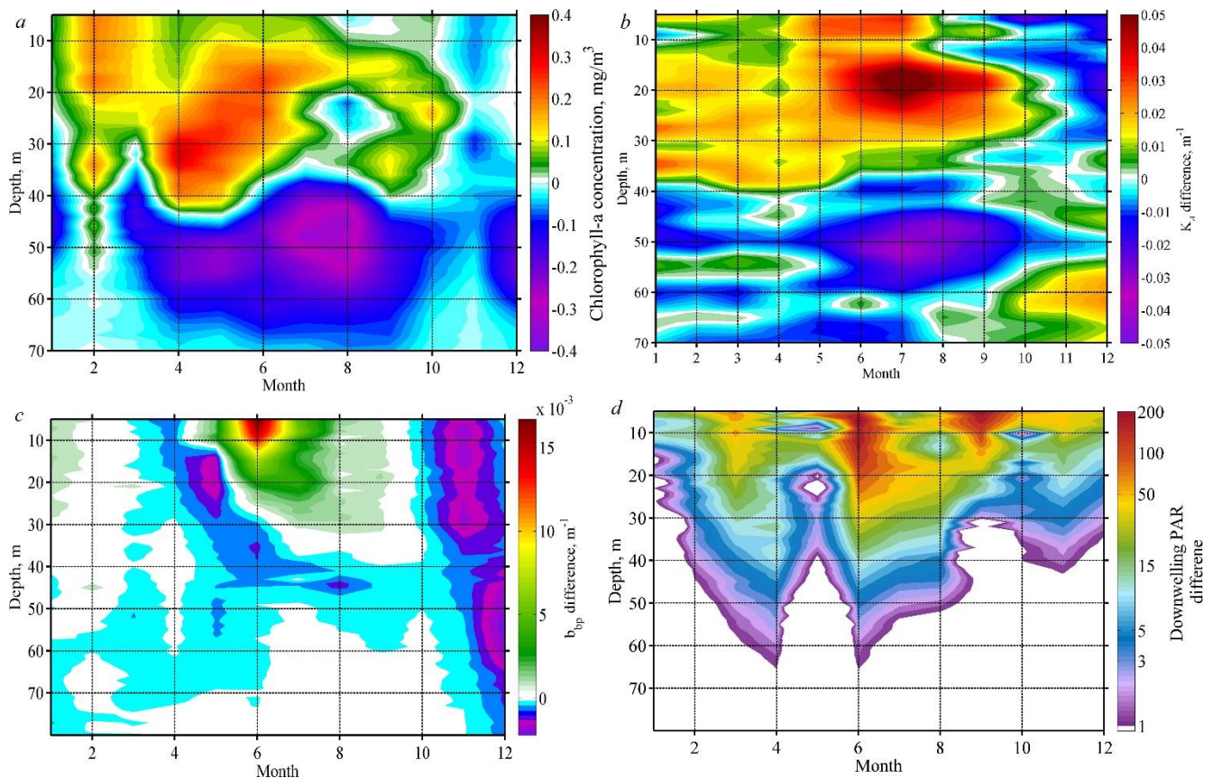
(New) Figure 6: Seasonal diagram of a difference of vertical distribution of Chl (a), K_d ( m^{-1} ) (b), b_{bp} ( m^{-1} ) (c) between 2017 and 2016. Difference in PAR ( \mu mol photons m^{-2} s^{-1} ) distribution between 2016 and 2017 (d).
