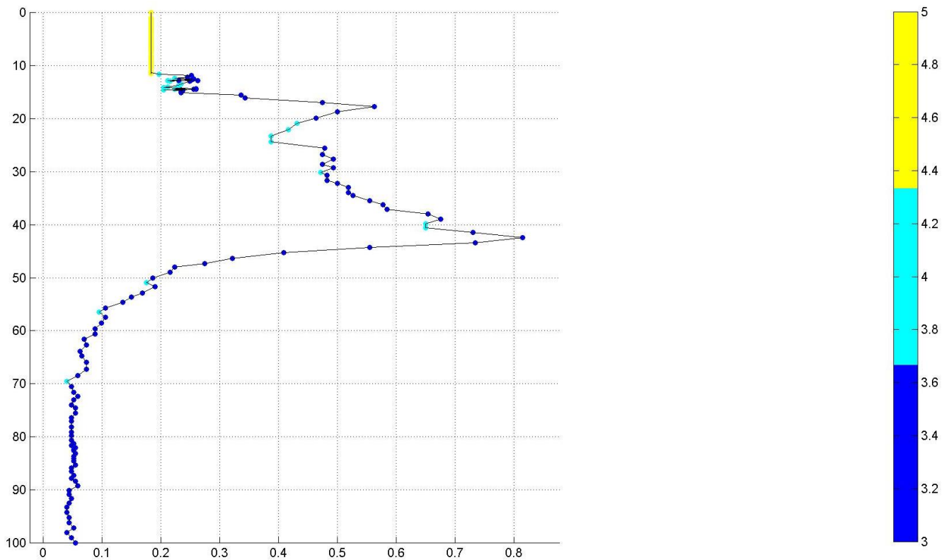
Fig. R2. Example of Chl profile for 31 August 2020 with QC flags shown by colors.
