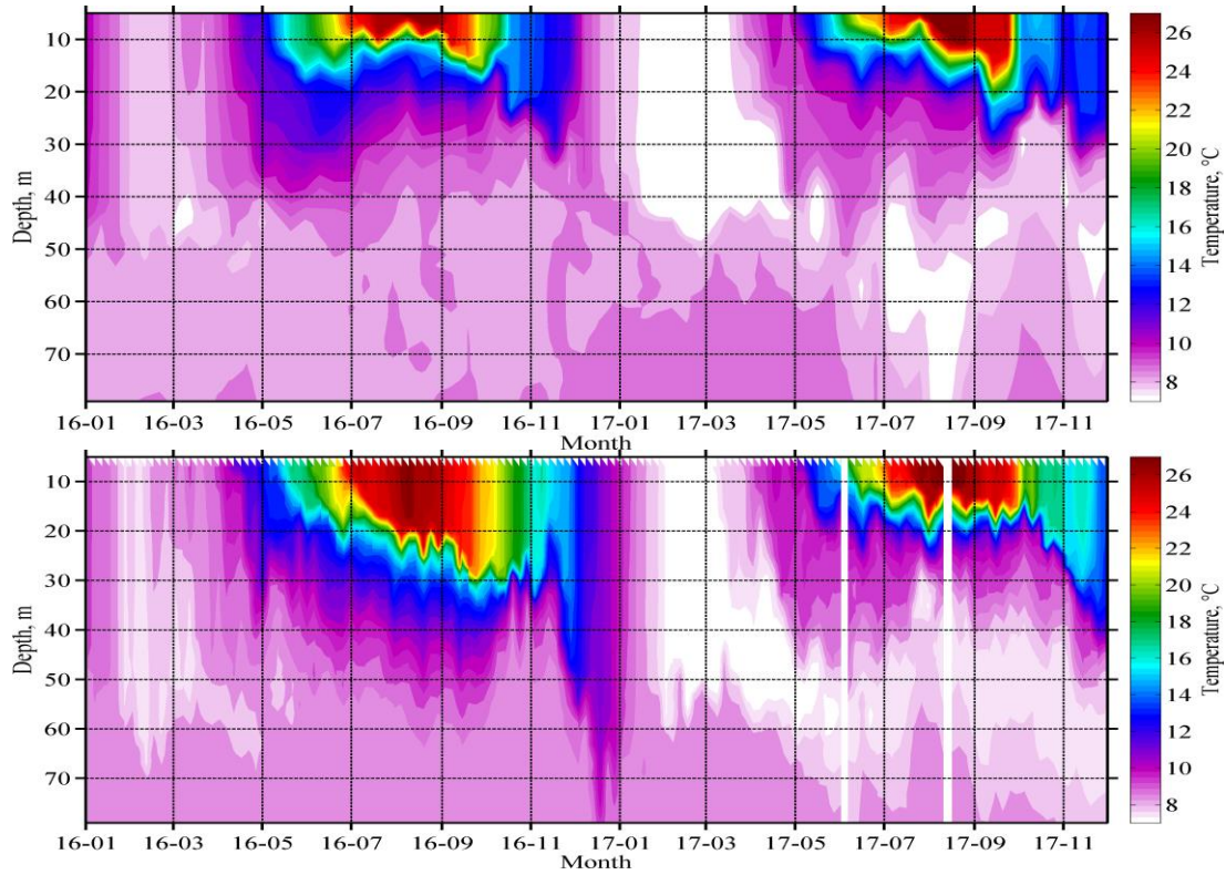
Fig. R4. Time variability of temperature according to measurements of the float #7900591(top) and float #6901866 (bottom)
