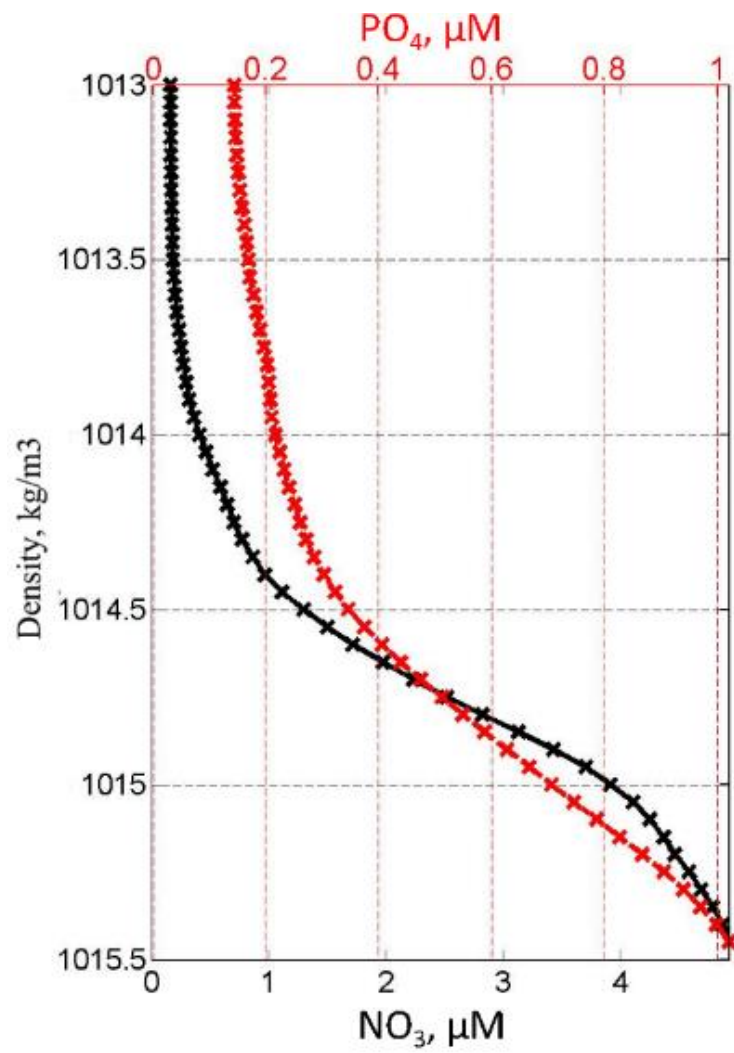
Supplementary Fig. S1. The multi-annual average vertical profiles of nitrate (NO 3 ) and phosphate (PO 4 ) in \sigma -coordinates for October, the month preceding the onset of intense winter convection.
