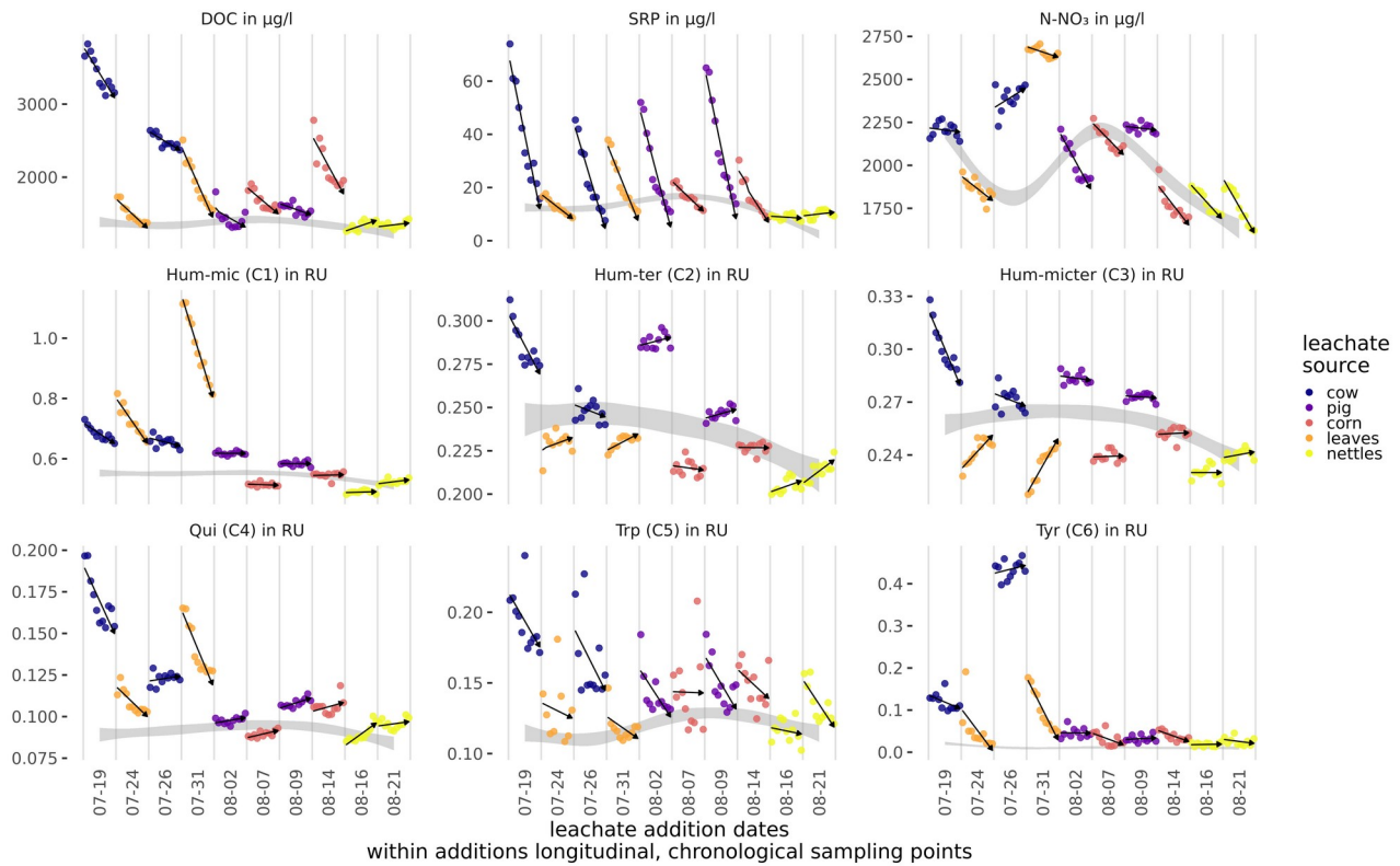
Figure 4: Measured concentrations of DOC, SRP, and N-NO 3 , and Raman units (RU) of DOM fractions along the stream course for the different samplings. The values are corrected for dilution effects. (see also Table S1). Arrows show the general trend of the concentrations/RUs from up- to downstream. The ambient concentrations were interpolated from measurements taken in-between leachate additions and are visualized as grey ribbons (see Table S1 for ambient conditions and additional amounts from leachate additions at the upstream station).
