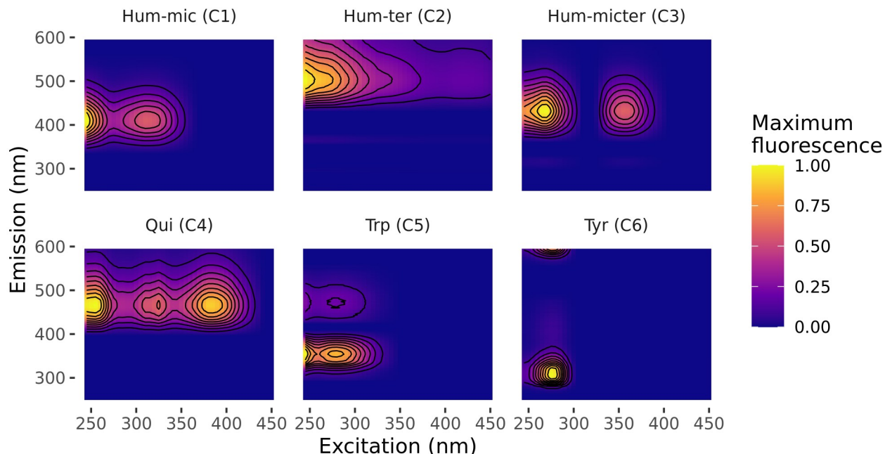
Figure 3: Fluorescence spectra of the identified PARAFAC components.
