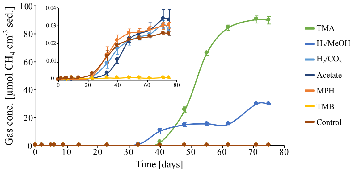
525 Figure 5: Methane production in batch incubations of peat sediment slurries , where, CH 4 is expressed as CH 4 cm -3 of original peat sediment over the course of 75 days. Substrates: trimethylamine (TMA), hydrogen and methanol (H 2 /MeOH), hydrogen and CO 2 (H 2 /CO 2 ), acetate, methoxyphenol (MPH), trimethoxybenzoate (TMB), and an anaerobic control incubation without substrate amendment (Control). Data points represent the average of triplicate measurements on triplicate incubations. Error bars indicate the standard deviation of the mean. The insert depicts a zoom in on the CH 4 concentrations excluding the incubations on TMA and H 2 /MeOH.
