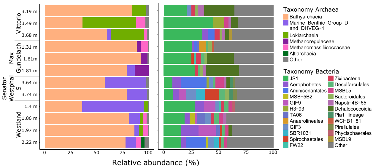
555 Figure 6: Phylogenetic classification of amplified archaeal (left) and bacterial (right) 16S rRNA genes. The Y-axis values indicate the depth beneath sea floor (dbfs). The maximum taxonomy depth is on family level. Taxonomic groups with < 2% abundance are grouped in 'Other'.
