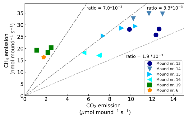
Figure 3. Mound CO 2 emissions ( \mu\text{mol mound}^{-1} \text{s}^{-1} ) versus mound CH 4 emissions ( \text{nmol mound}^{-1} \text{s}^{-1} ). Dotted lines indicate the different d\text{CH}_4/d\text{CO}_2 emission ratios.
