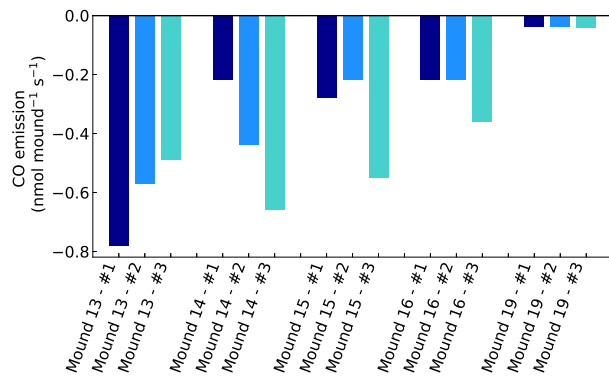
Figure A1. CO emissions of valley mounds nr. 13 -19, expressed in \text{nmol mound}^{-1} \text{s}^{-1} , which represents a collar area of 0.25 \text{ m}^2 . All mounds were measured 3 times during one week, and each series-nr (#) was measured on the same day and in the same order.
