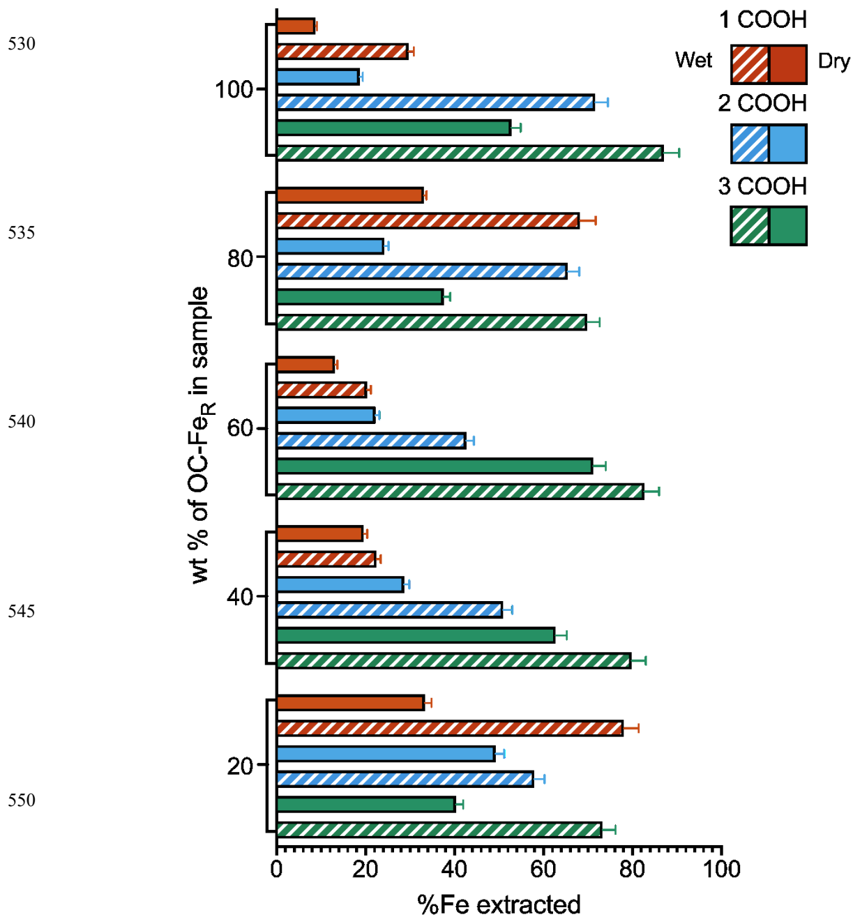
555 Figure 2: Fe recovery from freeze-dried vs slurry coprecipitates. Solid bars show dried samples while patterns show the wet (slurry) samples. 1/2/3 COOH refers to the number of carboxyl groups present in the coprecipitated organic acids. Each error bar shows maximum compound error.
