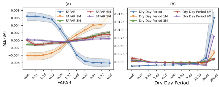
Fig. 9. First-order ALEs for different antecedent (< 1 yr) relationships with (a) FAPAR and (b) dry-day period (DD) in the 15VEG_FAPAR model, showing the underlying relationships with BA.
