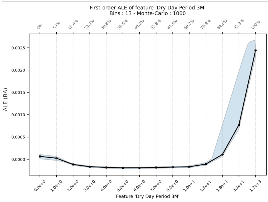
Fig. 6. First-order ALE plot showing the effect of the 3-month antecedent dry-day period (DD 3M) on burnt area (BA) in the 15VEG_FAPAR_MON model after accounting for all other variables.
