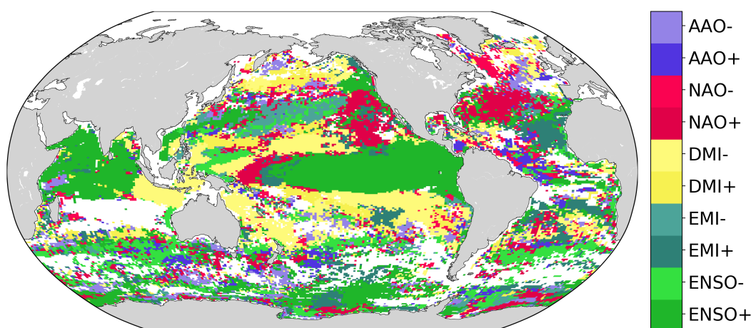
Figure 10. Phases of large-scale climate modes associated with the highest frequency of compound event days from 1998 to 2018. Regions for which the base frequency over the whole 1998-2018 period is <1% are marked white.
