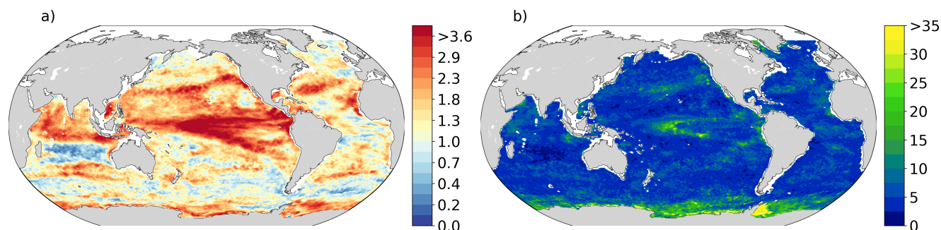
Figure 4. Observed frequency and duration of compound marine heatwaves and low chlorophyll extremes averaged over the 1998-2018 period. (a) Frequency of compound MHW and LChl event days (%). Note the nonlinear scale. Here, the frequency is equivalent to the likelihood multiplication factor. (b) 90th percentile of the duration of compound events.
