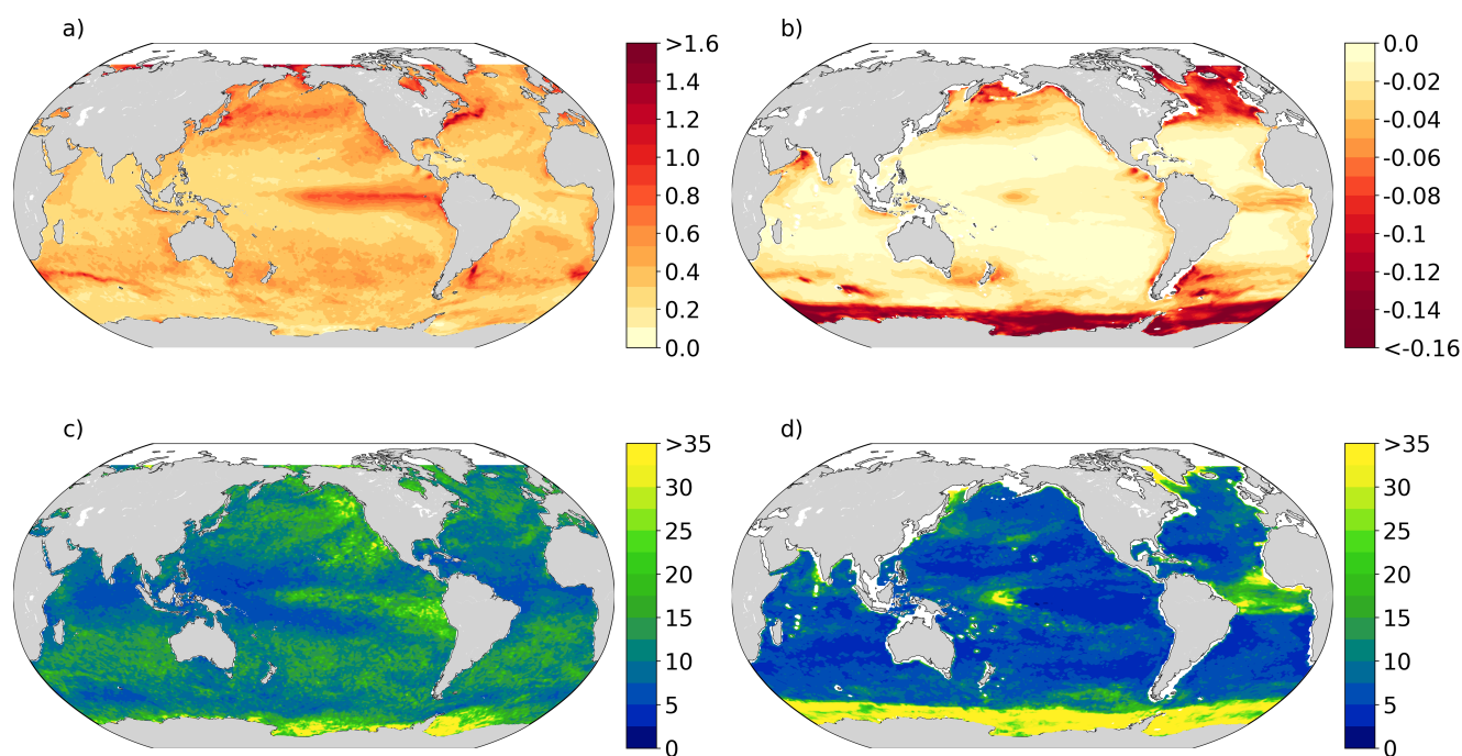
Figure 3. Observed marine heatwave and low chlorophyll extreme event characteristics averaged over the 1998-2018 period. (a,b) Mean intensity of MHWs (°C) and LChl events ( \text{mg m}^{-3} ). (c,d) 90th percentile of the duration of MHWs and LChl events in days.
