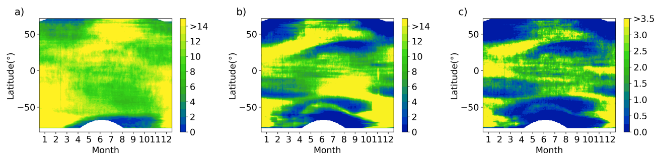
Figure 7. Seasonal cycle of MHWs, LChl events and compound events over the 1998-2018 period. Frequency of (a) MHW, (b) LChl and (c) compound event days (%) as a function of latitude and day of the year.
