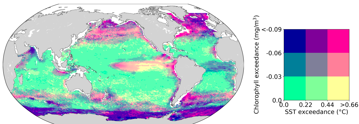
Figure 6. Intensity of compound marine heatwaves and low-chlorophyll events over the 1998-2018 period. Mean exceedance anomalies above the 90th and 10th percentile threshold of SST ( ^{\circ}\text{C} ) and chlorophyll ( \text{mg m}^{-3} ) anomalies, respectively, during compound events.
