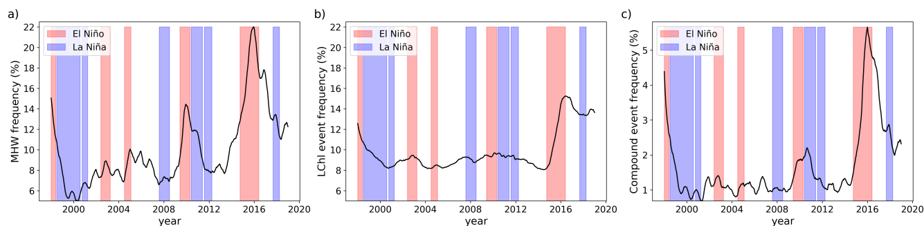
Figure 8. Global mean frequency of MHWs (a), LChl events (b) and compound events (c) over time. Daily time series are smoothed with a 1-year running mean to highlight interannual variability. Red and blue shadings indicate the occurrence of El Niño and La Niña events, respectively. These events occur when the El Niño 3.4 index exceeds 0.4 or is lower than -0.4, respectively, for at least 6 months. Note the different y-axes scales.
