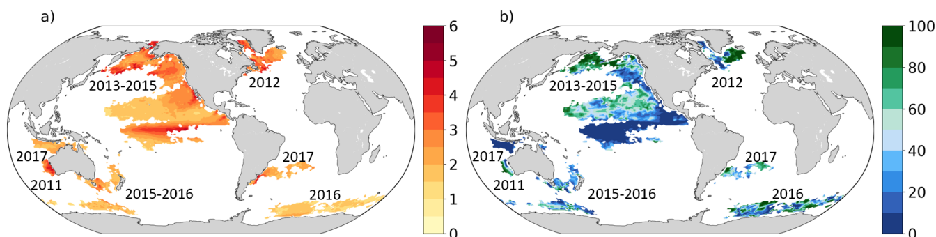
Figure 1. Recent (a) prominent large-scale marine heatwaves (MHWs) for which impacts have been documented, and (b) associated changes in surface chlorophyll concentrations ([chl]). We use sea surface temperature (SST) and [chl] deseasonalized anomalies. MHWs are defined when SST anomalies exceed their 99.5th percentile locally and numbers indicate the years of the MHW occurrences. (a) SST anomaly averaged over the MHWs duration. (b) Percentile associated with the mean [chl] anomaly averaged over the duration of the MHW, compared to the local empirical distribution of [chl] daily anomalies from 1998 to 2018. The MHWs extent is taken from Laufkötter et al. (2020) and corresponds to a spatiotemporally continuous area where each grid cell exhibits daily temperature anomalies above the 99.5th percentile.
