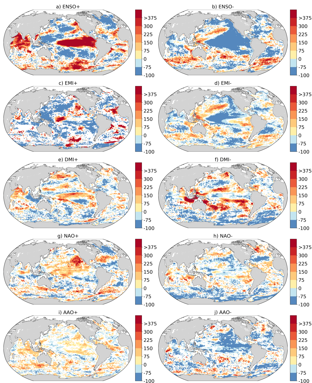
Figure 9. Frequency change in compound event days during positive and negative phases of several climate modes compared to their frequency over the complete 1998-2018 period (in %). Analyzed climate modes are: (a,b) El Niño Southern Oscillation, (c,d) El Niño Modoki, (e,f) Indian Ocean Dipole using its Dipole Mode Index, (g,h) North Atlantic Oscillation, and (i,j) Antarctic Oscillation. Grids cells where this frequency change is not statistically relevant remain white.
