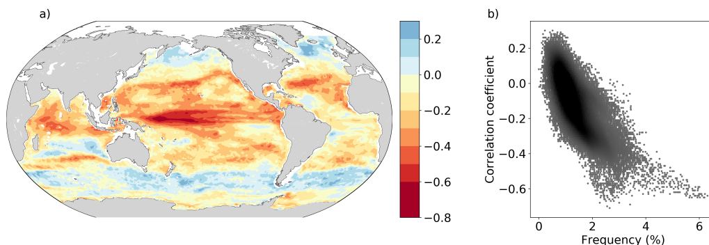
Figure 5. Correlation coefficient between SST and chlorophyll anomalies over the 1998-2018 period and its relationship to the occurrence of compound MHWs and LChl events. (a) Linear correlation coefficient between SST and chlorophyll anomalies. (b) Scatter plot of this correlation coefficient against the frequency of compound event days over the global ocean (see Fig. 4a).
