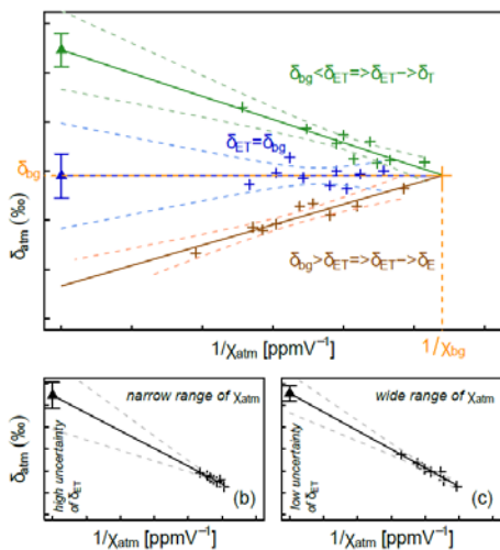
Figure 34. Illustration of the Keeling (1958) plot technique for determination of the isotopic composition of the surface flux, here evapotranspiration ( \delta_{\text{ET}} ). Subscript “bg” refers to the atmospheric background air, i.e., the air, which is not influenced by the surface ET flux. (a) Cases with different slopes of the regression line and implications for the nature of the surface flux: ET tends either toward transpiration (T) or evaporation (E). Illustration of the importance of the (narrow or wide) spread in water vapour mixing ratio ( \chi_{\text{atm}} , ppmV) values for the uncertainty of the \delta_{\text{ET}} estimate (panels b and c).
