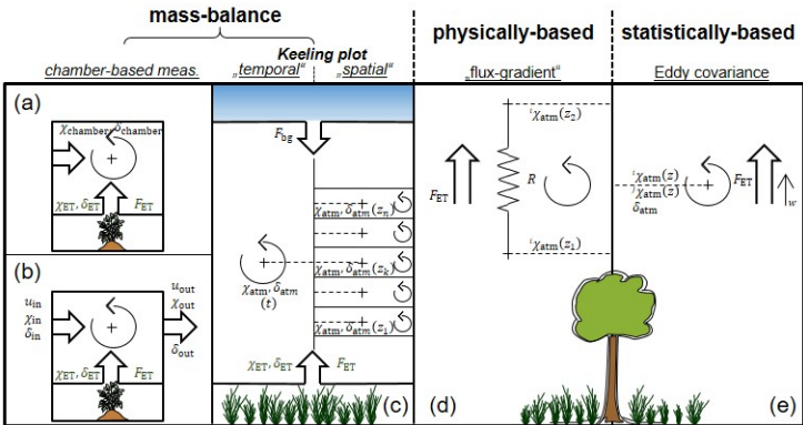
Figure 23. Summary of the different approaches (mass-balance, physically- and statistically-based) methods for determination of \delta_{ET} with the relevant variables and fluxes for each case.
