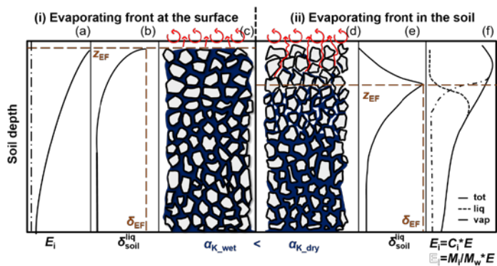
Figure 45. Effect of the water status of the soil, i.e., the positioning of the evaporating front (EF, dashed line), on the value of kinetic fractionation factor ( \alpha_K ). Panels a-c refer to the situation of a saturated soil (subscript “wet”) where the EF is located at the soil surface; panels d-f refer to a dry soil with the EF below the soil surface. The corresponding soil water total (solid line), liquid (dotted line), and vapour (dash-dotted line) isotopic flux profiles ( E_i , [M L -3 ]) (panels a/f), soil liquid isotopic composition profile (panels b/e) are reported as well. Adapted from Braud et al. (2005).
