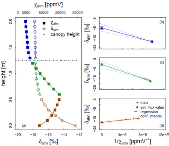
Figure 56. One example of application of the Keeling (1958) plot technique to synthetic data that would be collected with a field-deployable lift at high vertical resolution (0.1 m) (for implications on measurement frequency, which also needs to be high ( \geq 5 Hz), see sections 3.1 and 4 of Ney and Graf (2018)). The oxygen isotopic compositions of evapotranspiration, transpiration, and evaporation are estimated by the values of the y-intercepts of the linear regressions between the isotopic composition of the atmospheric water vapour ( \delta_{atm} ) and the inverse of the water vapour mixing ratio ( \chi_{atm} ) in three non-overlapping regions, i.e., (i) the “free atmosphere” (indicated by the blue symbols), (ii) the region spreading from the canopy height to the height of local maximum in \delta_{atm} (green symbols), and (iii) the region delimited by the \delta_{atm} local maximum height and the ground level (brown symbols). Also shown: 95 % confidence interval envelopes of the linear regressions (dashed lines) as well as error bars (1 standard error) of the y-intercepts.
