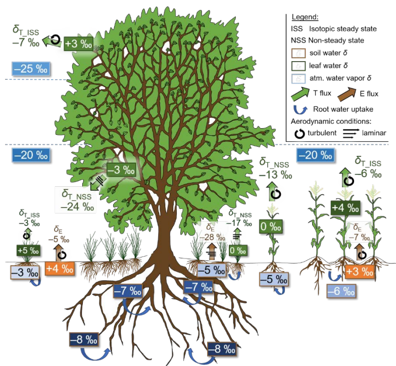
870 Figure 1: Conceptual drawing reporting the sources of differences in (synthetic) values between the (exemplary oxygen) isotopic compositions of evaporation ( \delta_E [‰]) and transpiration ( \delta_T [‰]) in an agroforestry context, namely (i) the type of vegetation and 875 root development (tree vs. maize crop vs. grass layer), (ii) the prevalence of isotopic steady state (ISS) or non-steady state (NSS) conditions for leaf water, and (iii) the environmental conditions acting on fluxes, i.e., soil water and atmospheric water vapour isotopic composition profiles, and leaf water isotopic composition (values displayed in brown, blue, and green outlined boxes). \delta_E and NSS \delta_T values were calculated with the Craig and Gordon (1965) model assuming laminar flow conditions (designated by the three superimposed arrows) under the pictured tree and within its canopy and fully turbulent conditions (designated by a circular arrow) elsewhere (e.g., at the top of the tree canopy, and above the maize crop for \delta_T and in its interrow space for \delta_E ).
