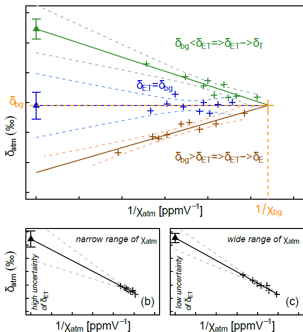
890 Figure 4. Illustration of the Keeling (1958) plot technique for determination of the isotopic composition of the surface flux, here evapotranspiration ( \delta_{\text{ET}} ). Subscript “bg” refers to the atmospheric background air, i.e., the air, which is not influenced by the surface ET flux. (a) Cases with different slopes of the regression line and implications for the nature of the surface flux: ET tends either toward transpiration (T) or evaporation (E). Illustration of the importance of the (narrow or wide) spread in water vapour mixing ratio ( \chi_{\text{atm}} , ppmV) values for the uncertainty of the \delta_{\text{ET}} estimate (panels b and c).
