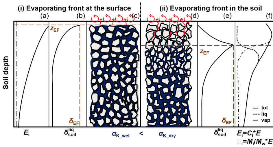
900 Figure 5. Effect of the water status of the soil, i.e., the positioning of the evaporating front (EF, dashed line), on the value of kinetic fractionation factor ( \alpha_K ). Panels a-c refer to the situation of a saturated soil (subscript “wet”) where the EF is located at the soil surface; panels d-f refer to a dry soil with the EF below the soil surface. The corresponding soil water total (solid line), liquid (dotted line), and vapour (dash-dotted line) isotopic flux profiles ( E_i , [M L -3 ]) (panels a/f), soil liquid isotopic composition profile (panels b/e) are reported as well. Adapted from Braud et al. (2005).
