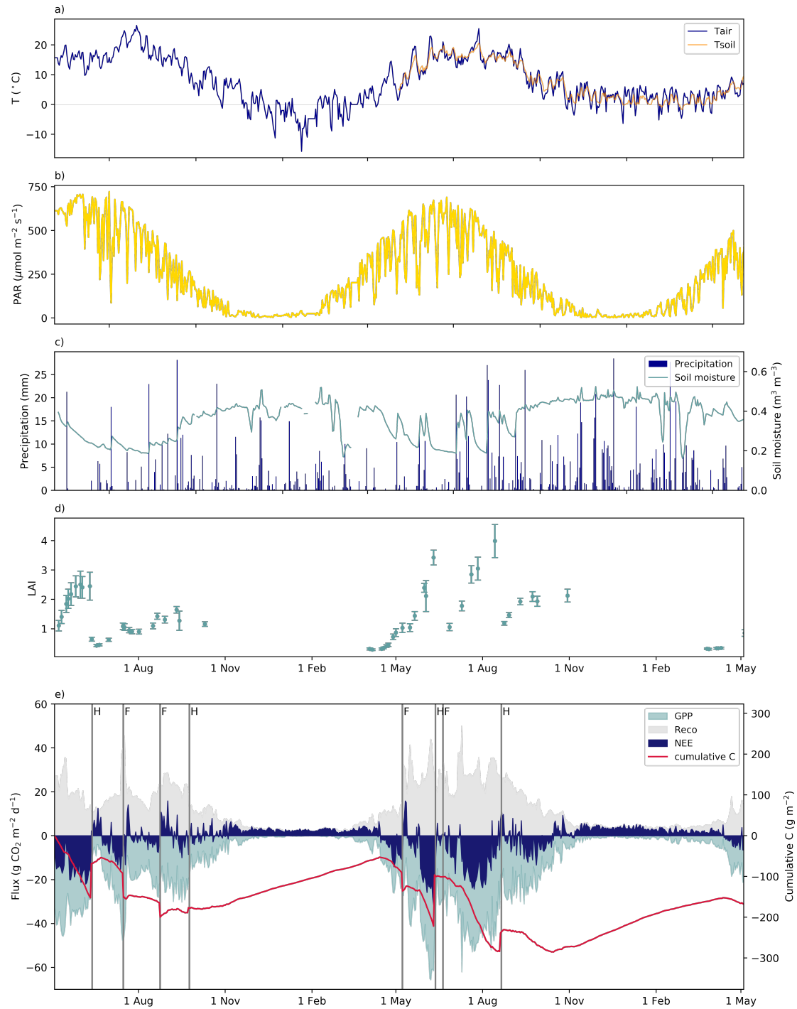
Figure 4. Daily mean a) air and soil (depth = 0.05 m) temperature, b) photosynthetically active radiation (PAR), c) precipitation and soil moisture (depth = 0.1 m), d) phytomass (PI) and leaf area indices index (LAI), and e) daily mean NEE, GPP, R_{eco} and cumulative carbon flux from May 2018 to May 2020.
