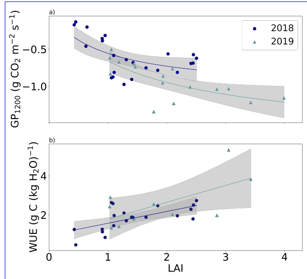
Figure 5. a) Daily photosynthetic capacity ( GP_{1200} ) and b) water use efficiency (WUE) as a function of leaf area index (LAI) during the two growing seasons. Grey areas represent the uncertainty estimation bands .
