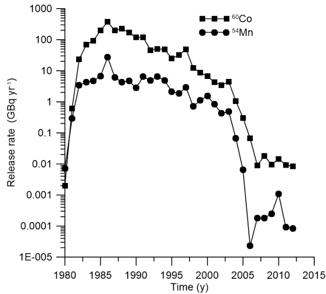
Figure 7. Release rates of 60 Co and 54 Mn according to measurements (Forsmark, 2014).
