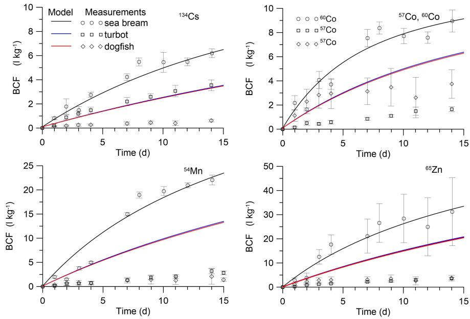
Figure 5. Simulated BCF in marine fish during the period of exposition in water. The simulations are compared with isotope measurements by Mathews and Fisher et al. (2008) in juvenile sea bream ( Sparus auratus ) and measurements by Jeffree et al. (2006) in turbot ( Psetta maxima ) and spotted dogfish ( Scyliorhinus canicula ).
