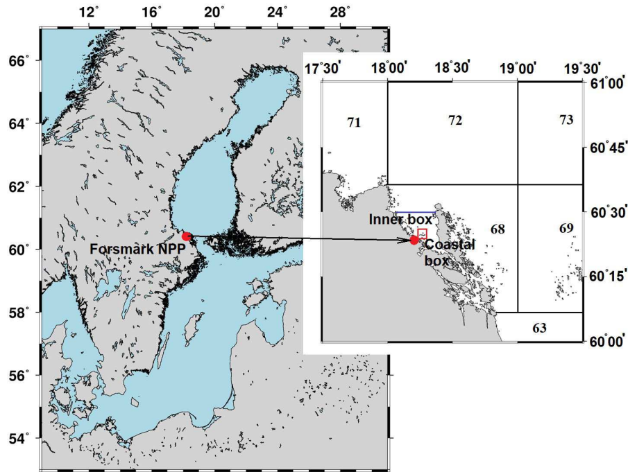
Figure 6. Compartment Box system around the Forsmark NPP. The numbers denote regional boxes in the box system of the Baltic Sea (Bezhenar et al., 2016). An additional “Inner box” is separated from regional box 68 by the blue line. The coastal box (red rectangle) surrounds the area, where cooling water from NPP is discharged.
