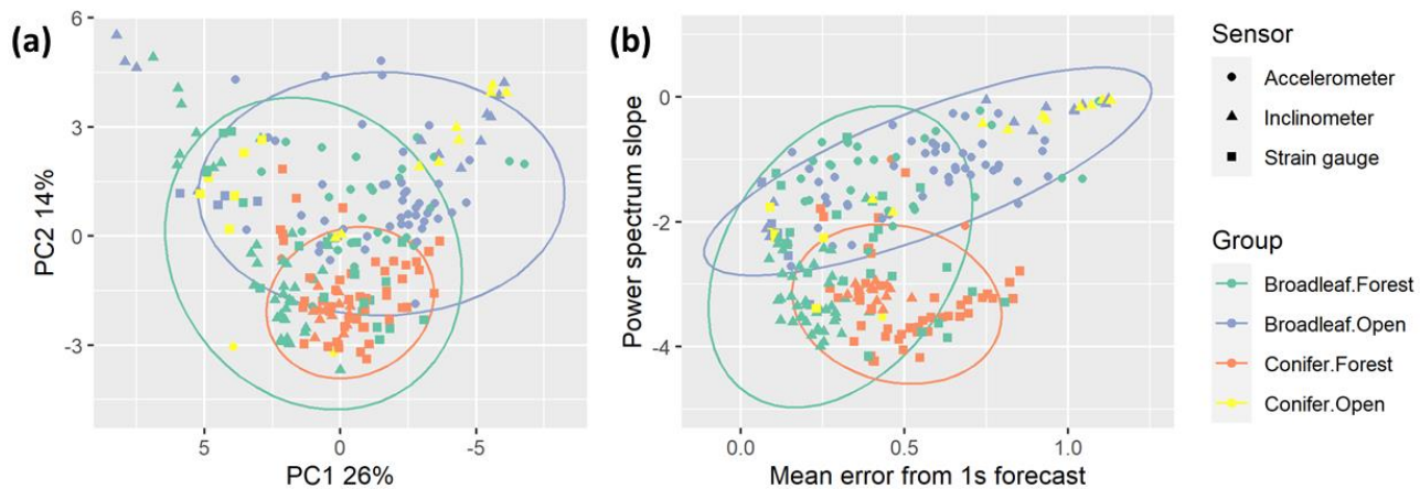
Figure 3 - Features of tree motion from 2259 trees during summer high (local) wind speed conditions projected on (a) first two principal component axes (arbitrary units) and (b) maximally discriminant axes (original units, unscaled). Ellipses represent Student's t-distributions around the data and were only drawn around groups with sufficient samples [broadleaf. forest (n=846), conifer. forest (n=635), broadleaf. open (n=63)].
