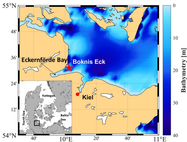
80 Figure 1: Location of the Boknis Eck Time-Series Station near the entrance of Eckernförde Bay in the southwestern Baltic Sea. The location map was created with the m_map package for Matlab R2019 (Pawlowicz, 2020).
