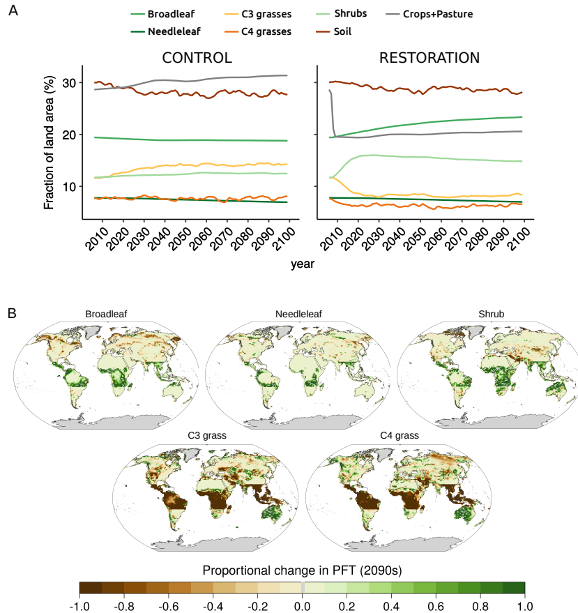
Figure 1. (A) Change in land cover 2006–2100 CE in control (left) and restoration (right) simulation. Urban (0.1%), inland water (1.9%), and ice fraction (9.7%) are constant and not included. Anthropogenic disturbance An anthropogenic land use mask is added on top of other land cover types, replacing woody PFTs with bare soil and preventing woody PFTs from replacing grassy PFTs, which include crops and pasture (see Methods 2.1.1). (B) Spatial difference in land cover in the restoration simulation relative to the control simulation over the 2090s.
