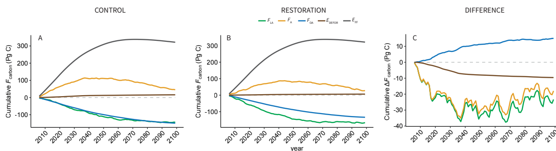
Figure 4. Effect of tropical land use stop and secondary succession on cumulative global carbon fluxes (2006–2100 CE) in (A) control and (B) restoration, and (C) cumulative difference between restoration and control simulation for land-atmosphere flux ( F_{LA} , green), ocean-atmosphere flux ( F_{OA} , blue), deforestation emissions ( E_{DEFOR} , brown), atmospheric carbon ( F_A , orange), and fossil fuel emissions ( E_{FF} , grey). The difference in fossil fuel emissions is zero and not plotted. Dashed line indicated zero, fluxes below zero indicate a carbon benefit in the restoration simulation w.r.t. the control simulation. Note the different vertical scales.
