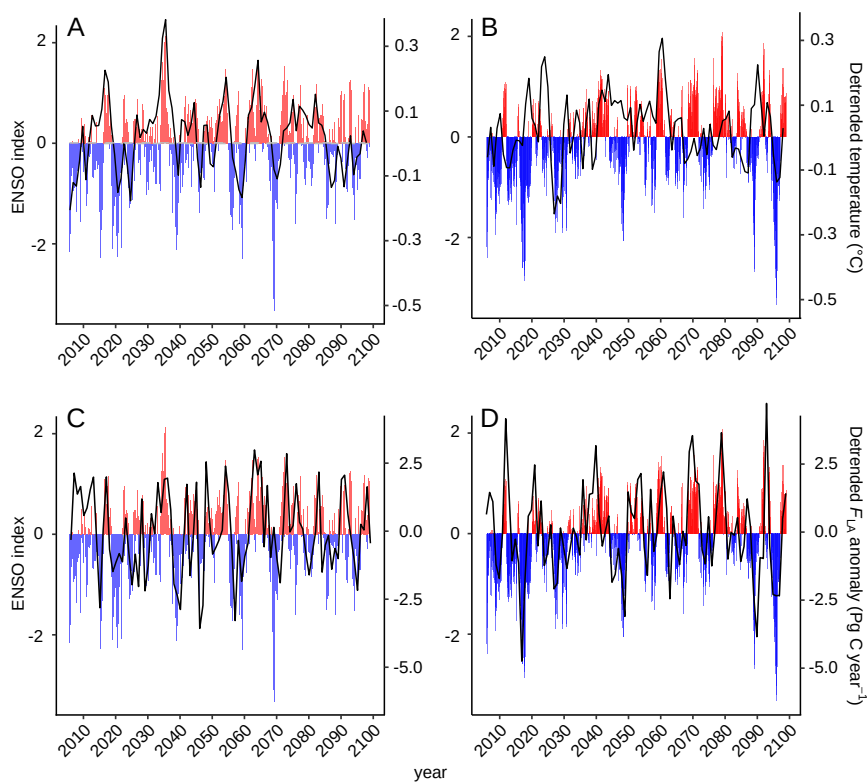
Figure A5. The impact of ENSO on global surface air temperature in the (A) control and (B) restoration simulation, and on the land carbon sink ( F_{LA} ) in the (C) control and (D) restoration simulation. Positive ENSO values represent El Niño events (red), negative values represent La Niña events (blue).
