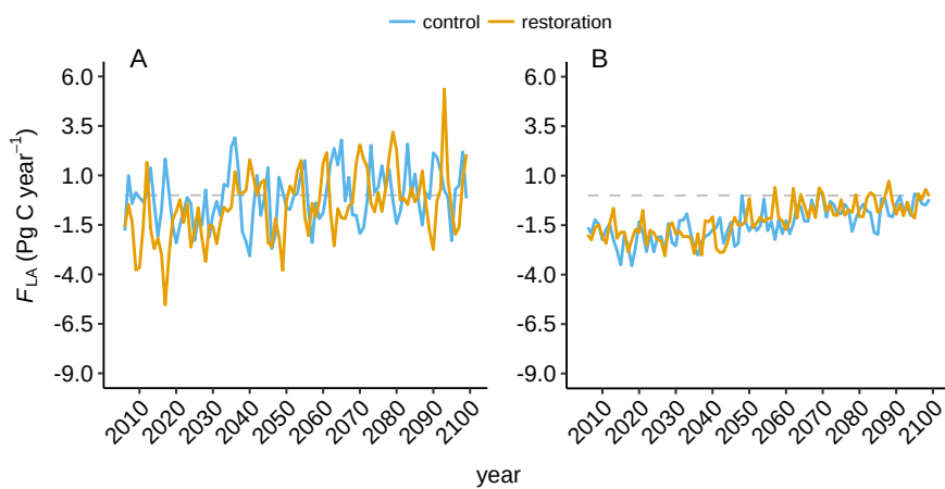
Figure A3. Tropical (A) and extratropical (B) land-atmosphere flux ( F_{LA} ) in the restoration (yellow) and control (blue) simulation.
