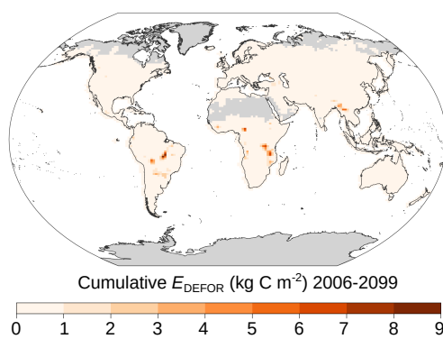
Figure A1. Hotspots of deforestation emissions in RCP 2.6. Cumulative deforestation emissions (2006–2099 CE) in the control simulation.
