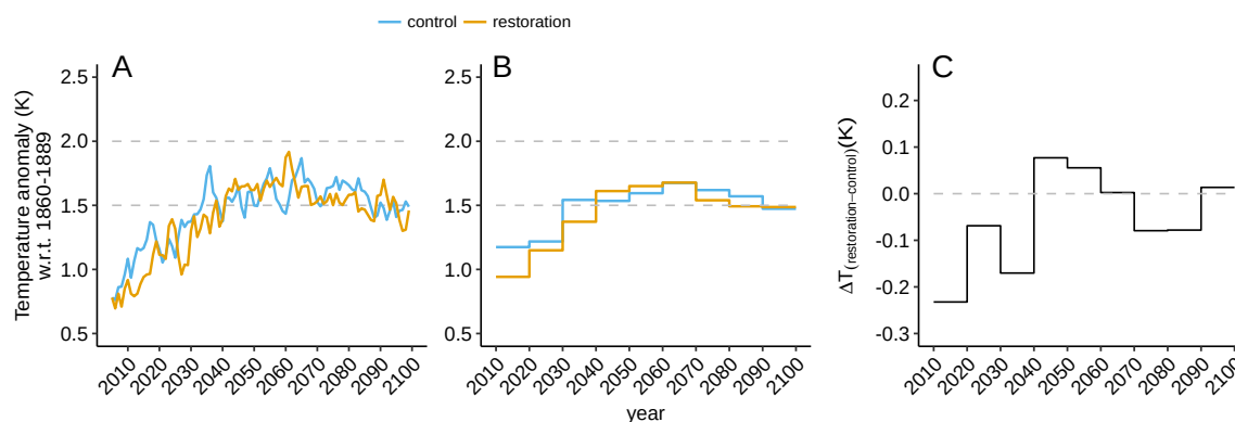
Figure 6. Global temperature time series showing (A) annual averages and (B) decadal averages for the restoration (yellow) and control (blue) simulation; (C) decadal difference between both simulations.
