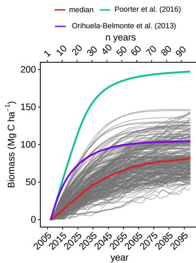
Figure A4. Aboveground biomass change in regenerating broadleaf forest in the restoration simulation. Modelled median increase (red) compared to observations (Orihuela-Belmonte et al., 2013; Poorter et al., 2016). Regenerating broadleaf forest are defined as grid cells with an increase in broadleaf PFTs of >30% of grid cell value.
