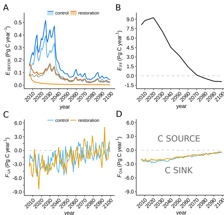
Figure 2. Modelled carbon emissions and fluxes 2006–2100 CE for the control run (blues) and restoration simulation (oranges). (A) Deforestation emissions ( E_{\text{DEFOR}} ), dark colours are global emissions, light colours are the tropics and dashed lines are emissions outside the tropics. (B) Prescribed fossil fuel emissions ( E_{\text{FF}} ) following RCP 2.6 (Liddicoat et al., 2013). (C) Global land-to-atmosphere flux ( F_{\text{LA}} ); (D) Global ocean-to-atmosphere flux ( F_{\text{OA}} ). Negative values represent a carbon sink. Note the different vertical scales.
