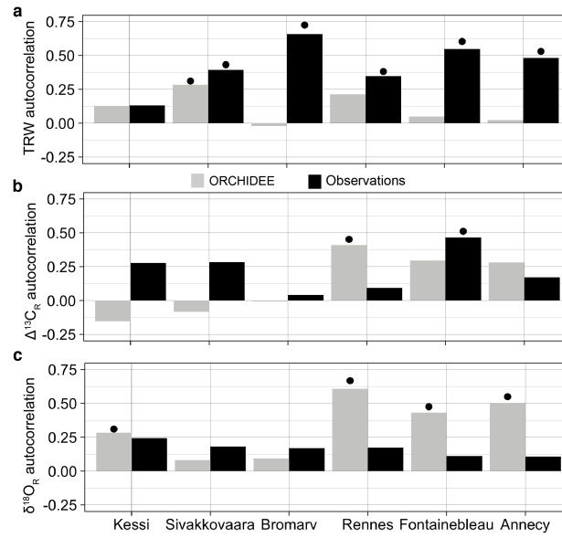
Figure 5. First-order autocorrelation in observed (black) and simulated (gray) tree-ring variables over the period 1960–2000. a Tree-ring width. b \Delta^{13}\text{C}_r . c \delta^{18}\text{O}_r . For Annecy the period of analysis is 1971–2000. Significance at the 95% confidence level is indicated by the black dots.
