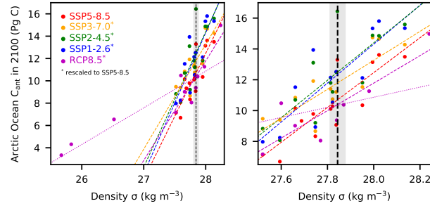
Figure 6. Arctic Ocean C_{ant} inventory in 2100, rescaled to SSP5-8.5 atmospheric C_{ant} concentrations (see Methods), against maximum Arctic Ocean sea surface density (95 th percentile) for SSP1-2.6 (blue; r^2=0.70 ), SSP2-4.5 (green; r^2=0.63 ), SSP3-7.0 (orange; r^2=0.70 ), SSP5-8.5 (red; r^2=0.72 ), and RCP8.5 (magenta; r^2=0.74 ) a ) over the entire density range and b ) over the density range from 27.5 to 28.3 \text{kg m}^{-3} . The simulated Arctic Ocean C_{ant} inventory in 2100 for each scenario (Fig. 2) was rescaled to SSP5-8.5 using the mean atmospheric C_{ant} concentration from 1850 to 2100 as a scaling factor. Linear fits use all available models for each scenario (dashed lines). For RCP8.5 an additional fit is shown excluding the three models with density anomalies below 27.5 \text{kg m}^{-3} b ) (dotted line; r^2=0.79 ).
