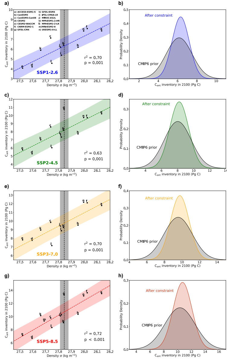
Figure 2. Emergent constraint on Arctic Ocean C_{\text{ant}} inventory in 2100. Maximum Arctic Ocean sea surface density (95 th percentile) and Arctic Ocean C_{\text{ant}} inventory in 2100 for 12-14 ESMs for a) SSP1-2.6 (blue), c) SSP2-4.5 (green), e) SSP3-7.0 (orange), and g) SSP5-8.5 (red). The ordinary least squares regressions (dashed lines) and the \pm one \sigma prediction intervals (shaded area) are shown for each SSP. Probability density functions before and after applying the emergent constraint for b) SSP1-2.6, d) SSP2-4.5, f) SSP3-7.0, and h) SSP5-8.5.
